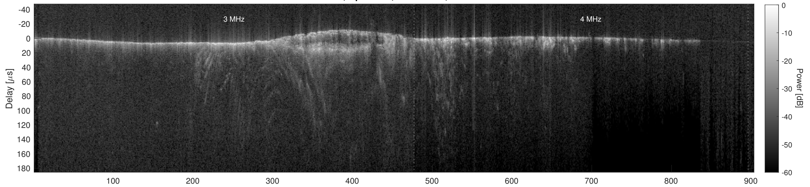
Orbit 15980, Cluttergram
