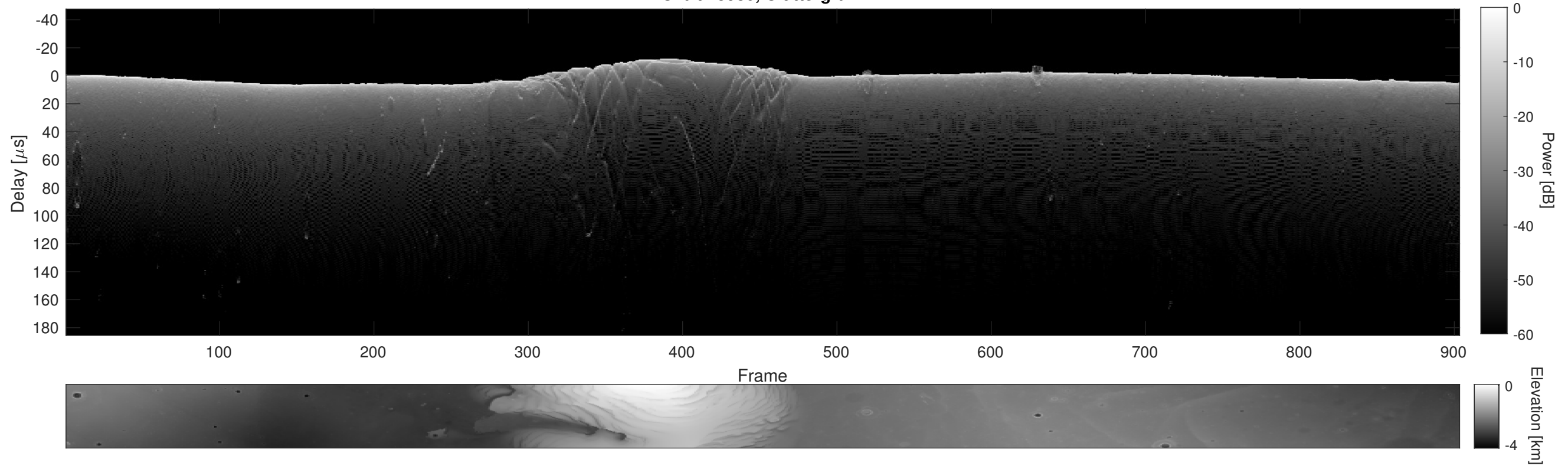
Orbit 15980, Cluttergram
