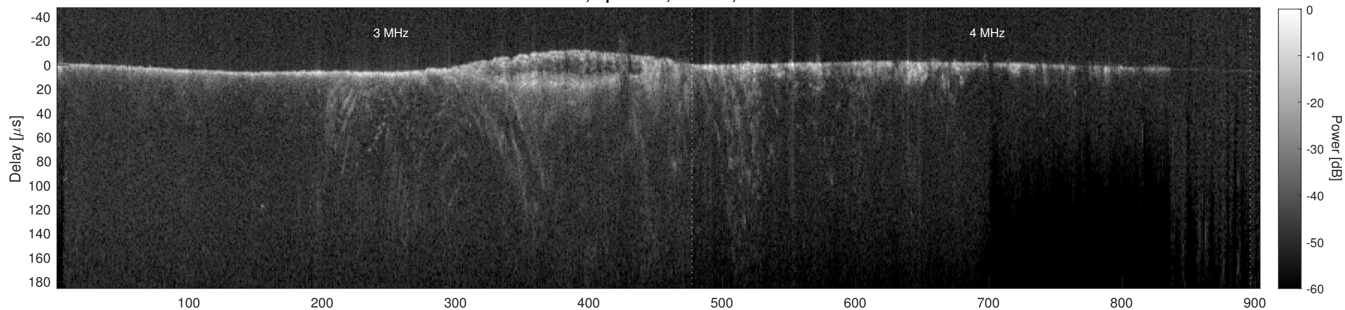
Orbit 15980, Cluttergram
