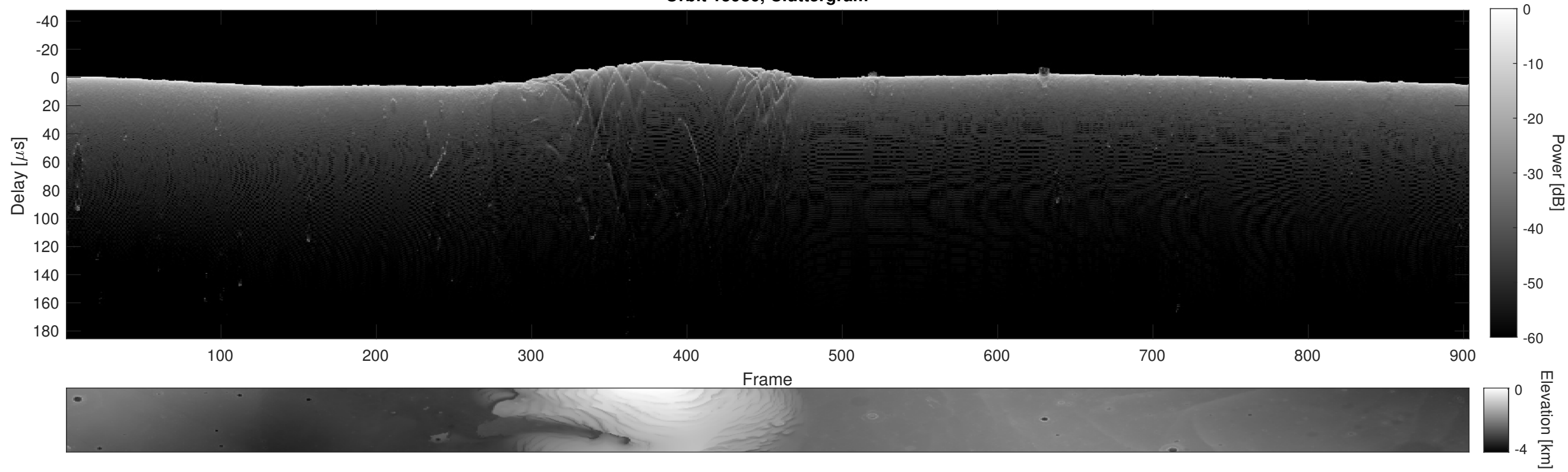
Orbit 15980, Cluttergram
