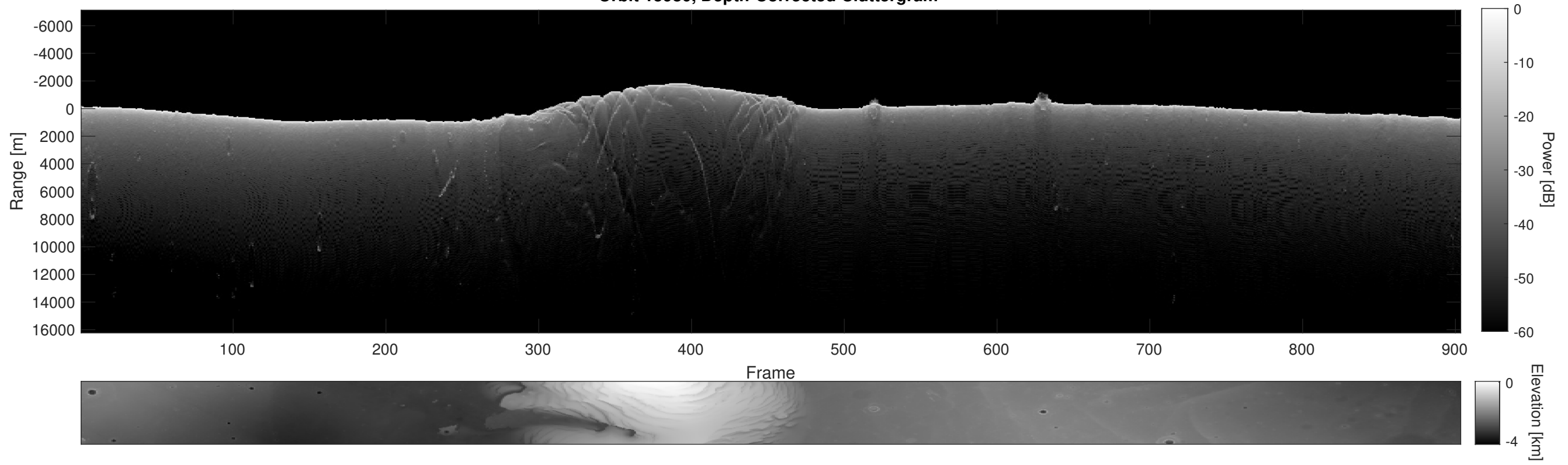
Orbit 15980, Depth-Corrected Cluttergram
