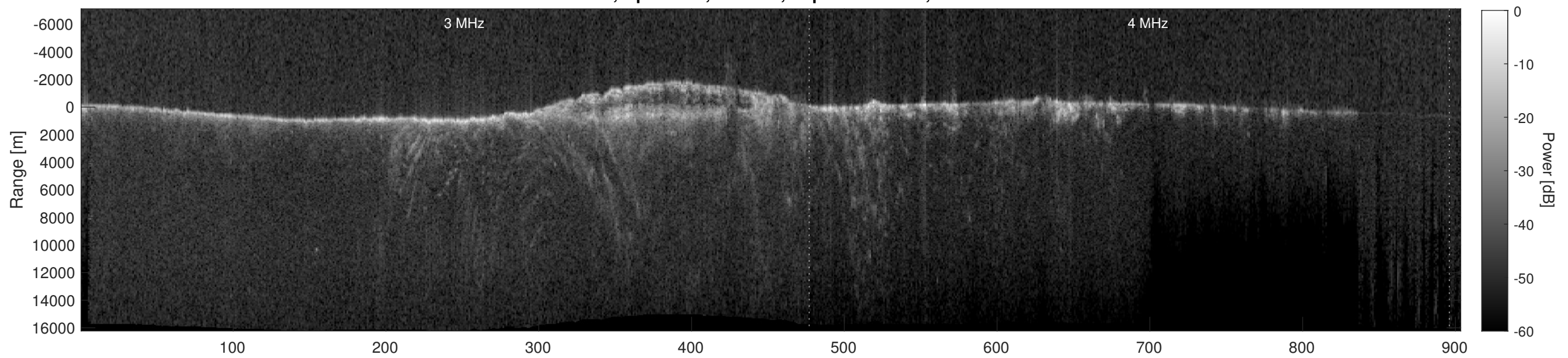
Orbit 15980, Depth-Corrected Cluttergram
