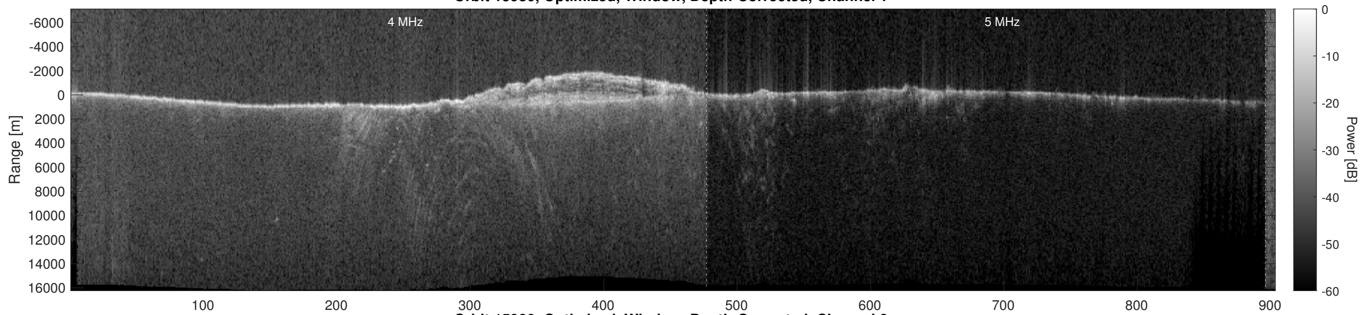
Orbit 15980, Optimized, Window, Depth-Corrected, Channel 2
