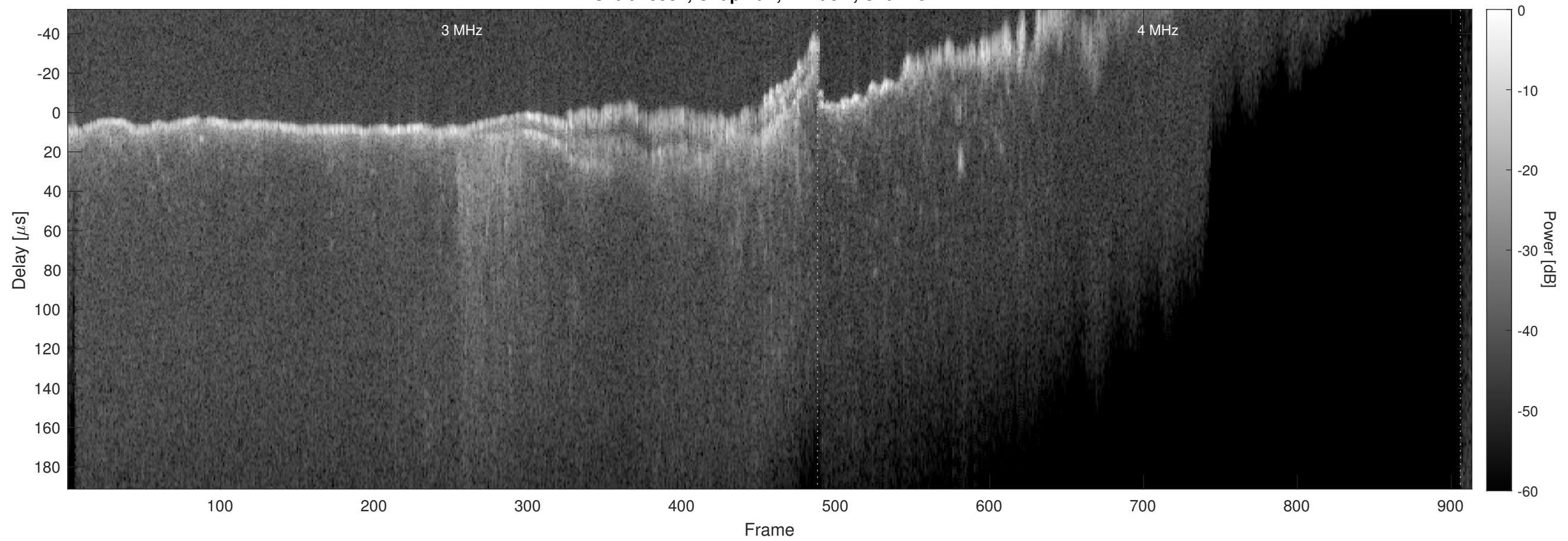
Orbit 15981, Chapman, Window, Channel 2
