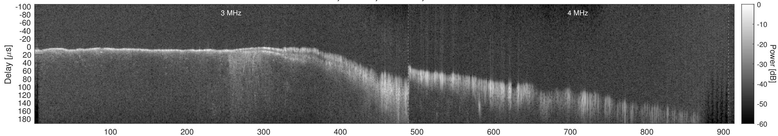
Orbit 15981, Window, Channel 2, Chapman
