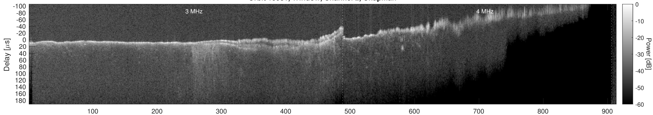
Orbit 15981, Window, Channel 2, Optimized
