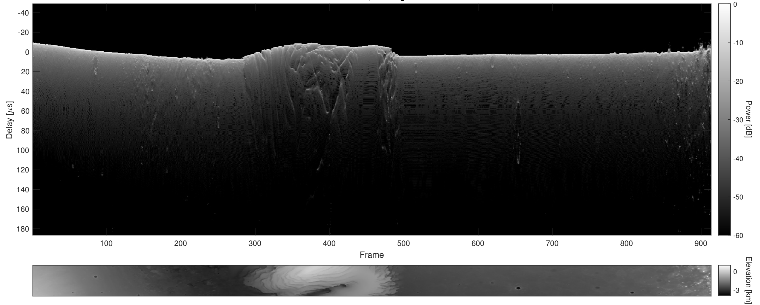
Orbit 15984, Cluttergram
