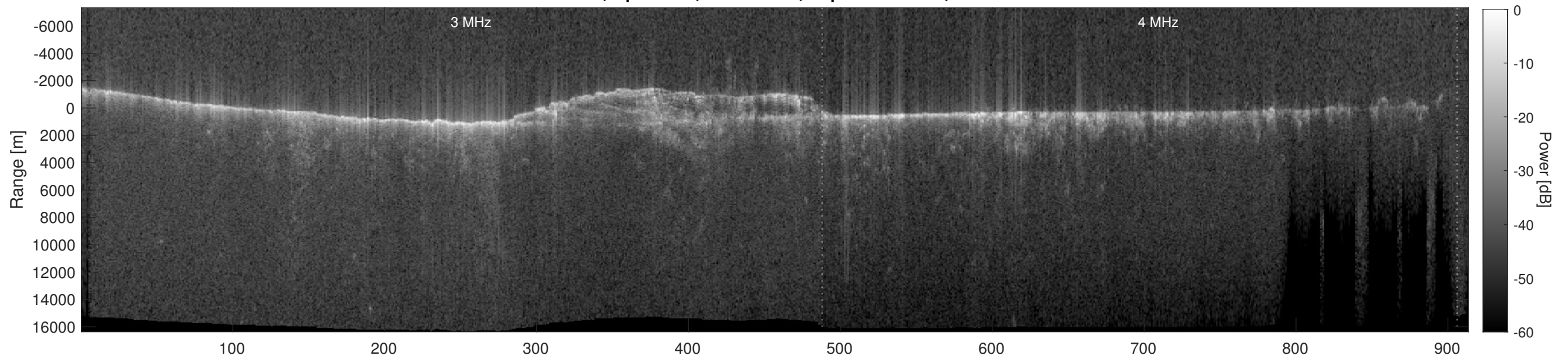
Orbit 15984, Depth-Corrected Cluttergram
