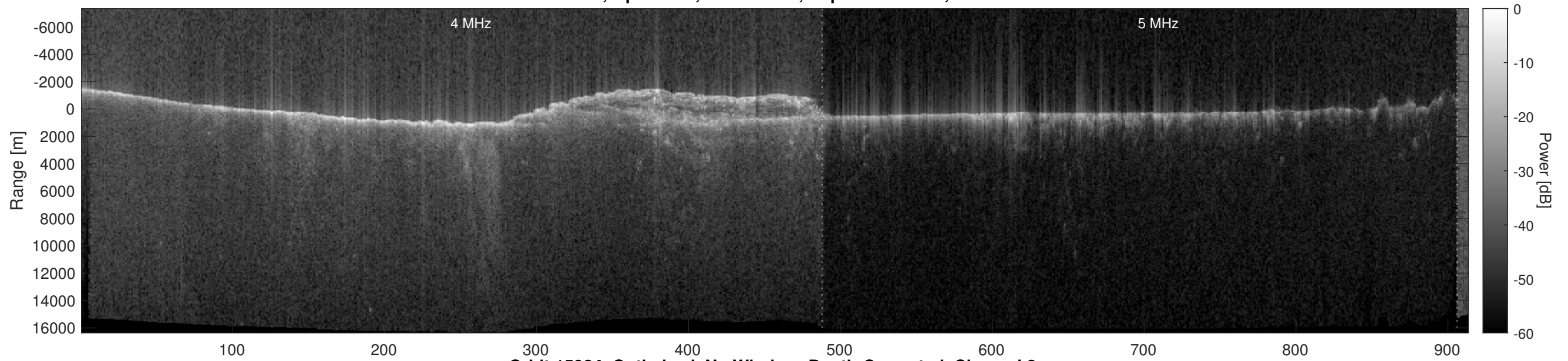
Orbit 15984, Optimized, No Window, Depth-Corrected, Channel 2
