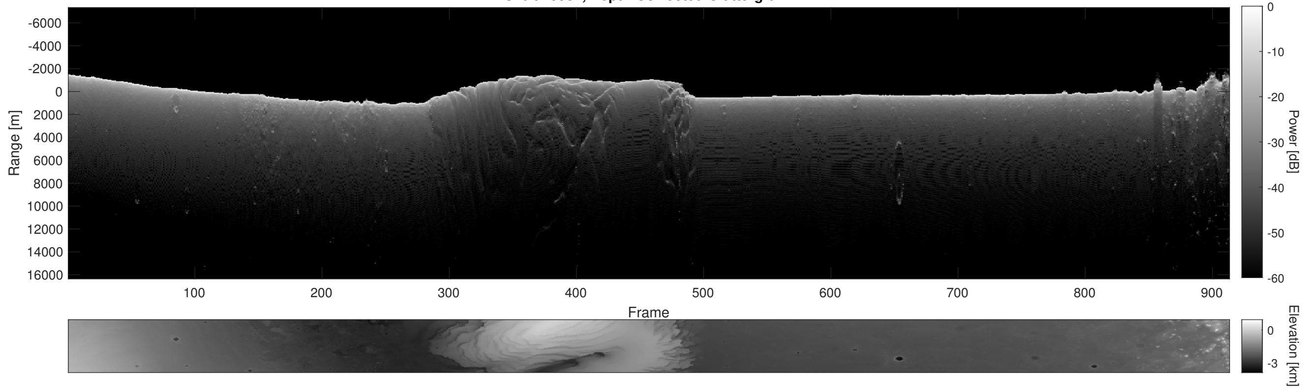
Orbit 15984, Depth-Corrected Cluttergram
