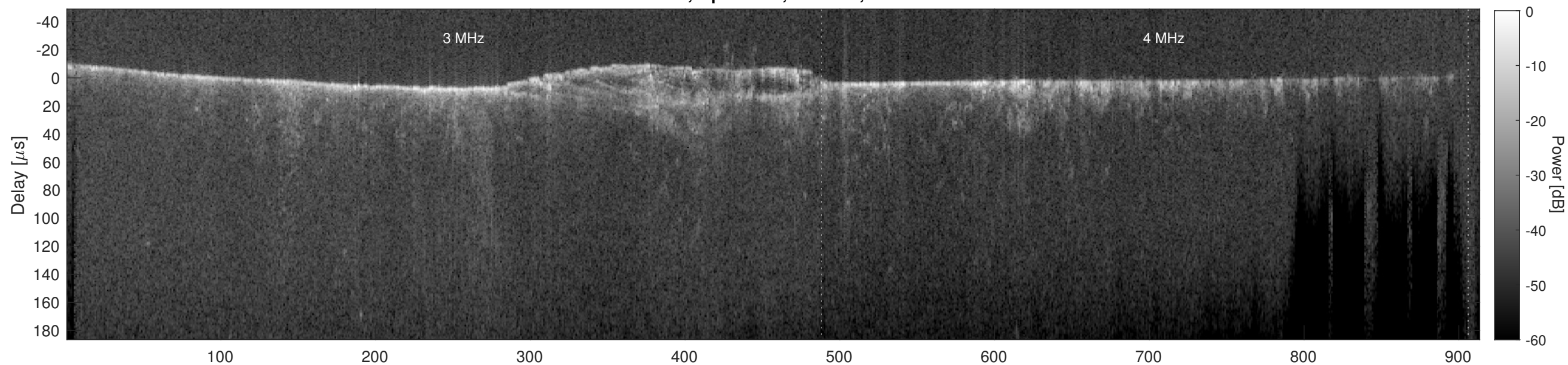
Orbit 15984, Cluttergram
