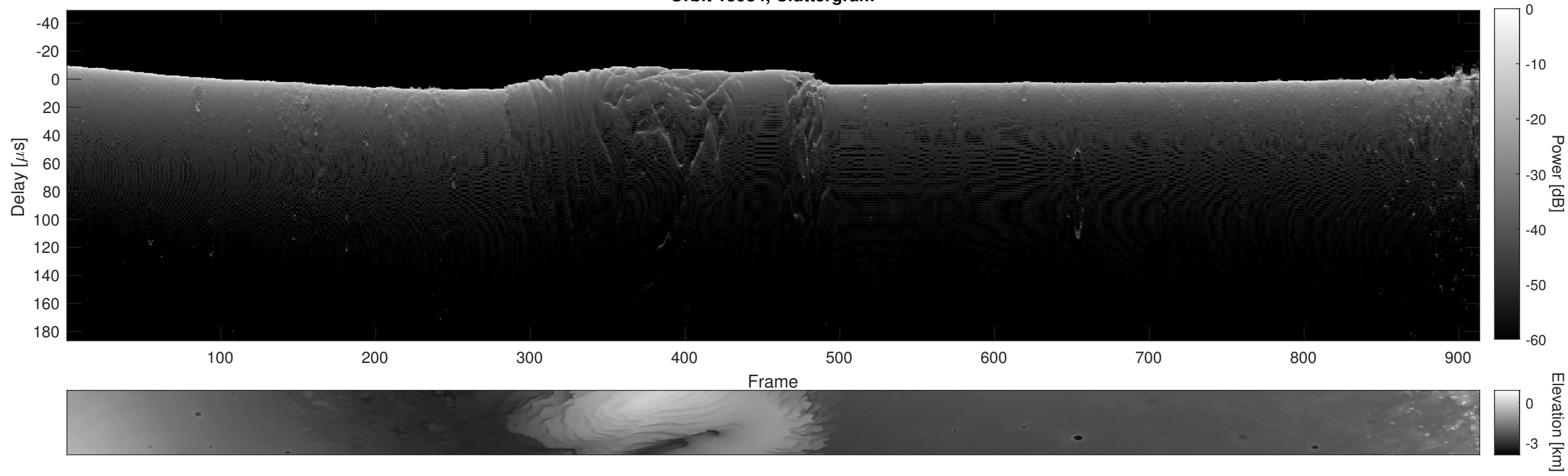
Orbit 15984, Cluttergram
