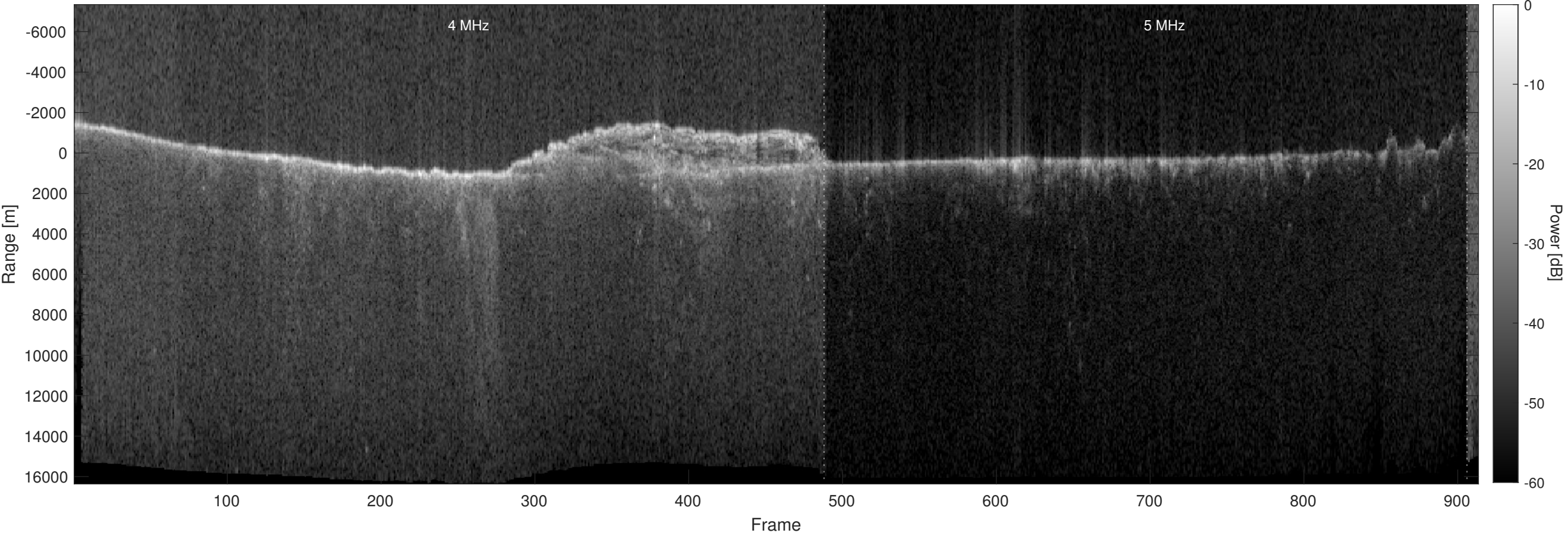
Orbit 15984, Optimized, Window, Depth-Corrected, Channel 2
