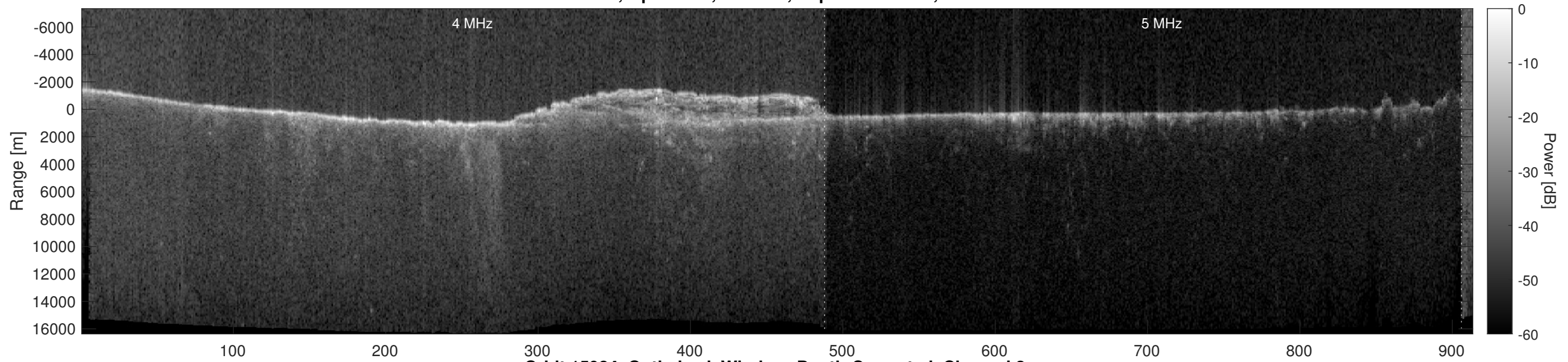
Orbit 15984, Optimized, Window, Depth-Corrected, Channel 2
