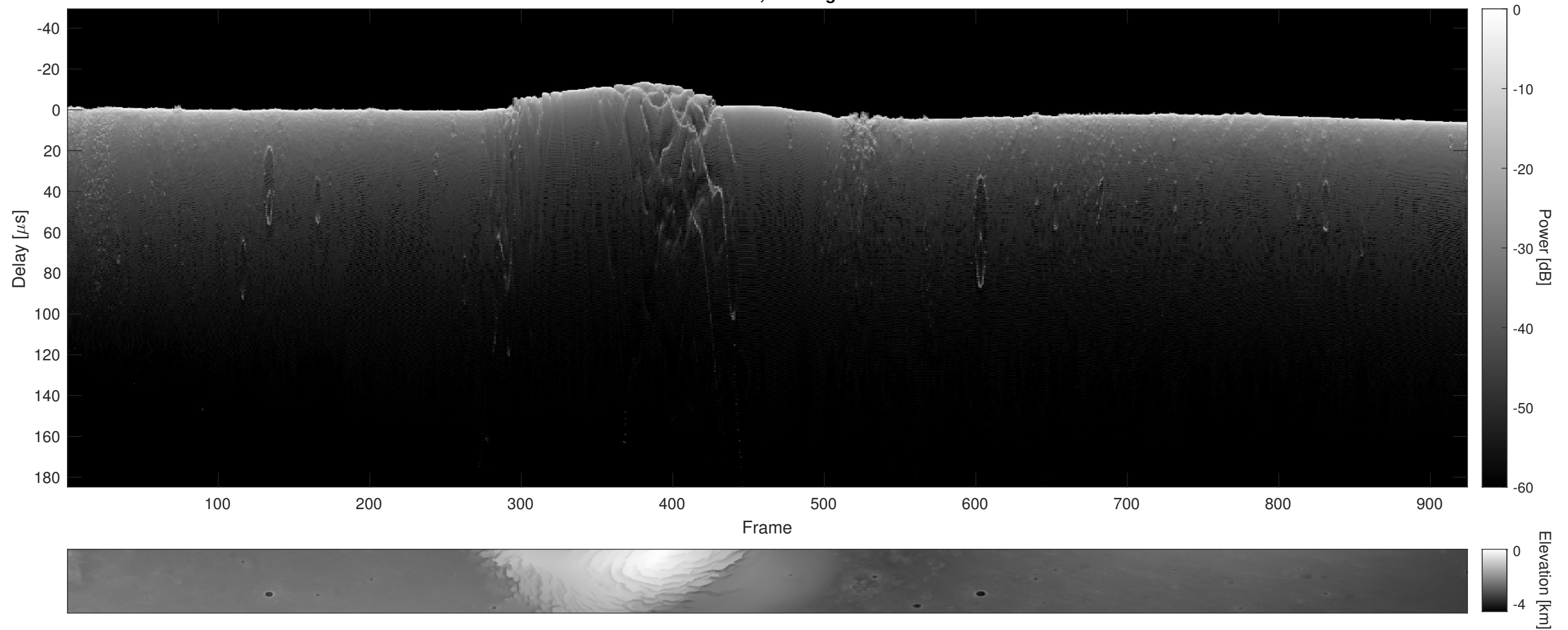
Orbit 15986, Cluttergram
