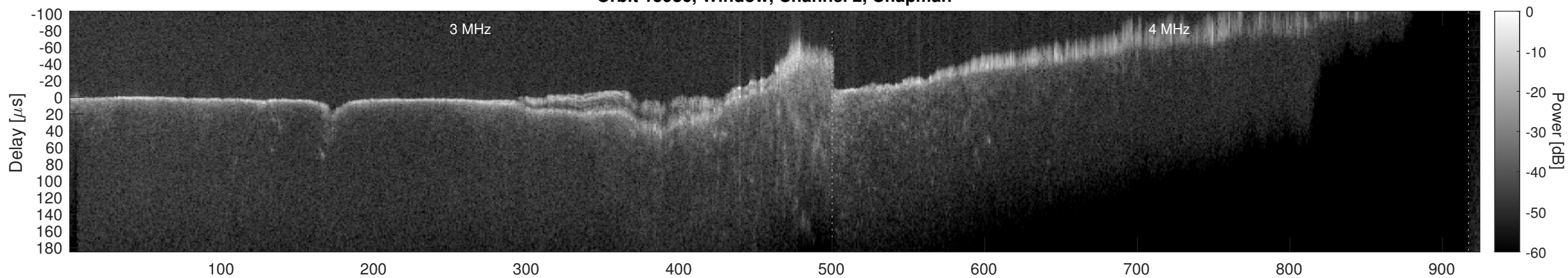
Orbit 15986, Window, Channel 2, Optimized
