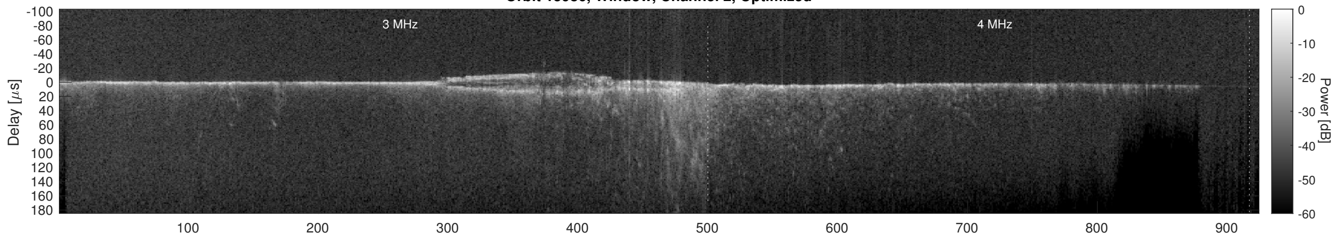
Orbit 15986, Cluttergram
