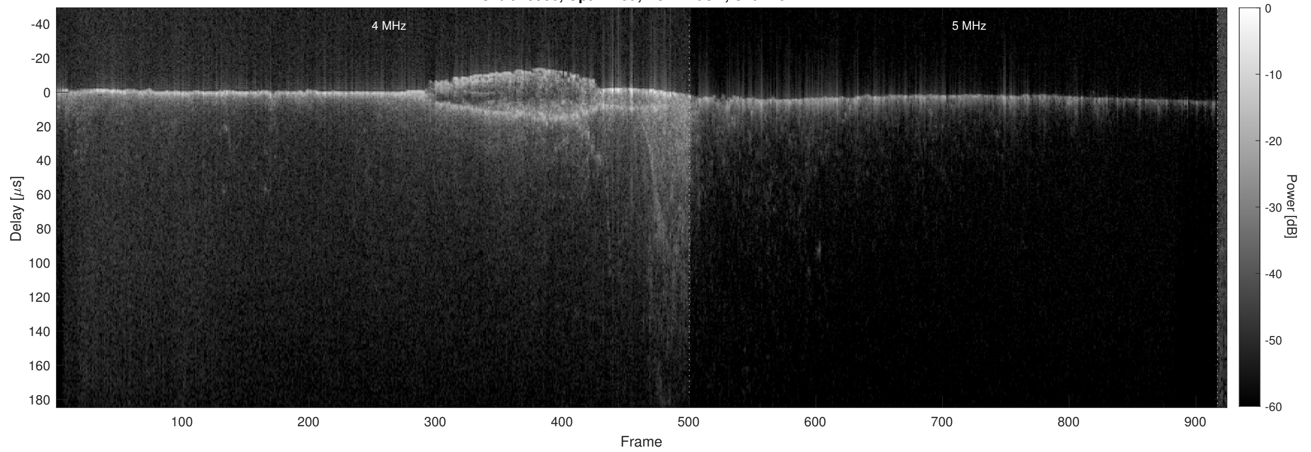
Orbit 15986, Optimized, No Window, Channel 2
