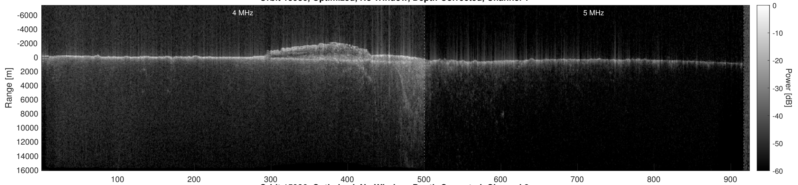
Orbit 15986, Optimized, No Window, Depth-Corrected, Channel 2
