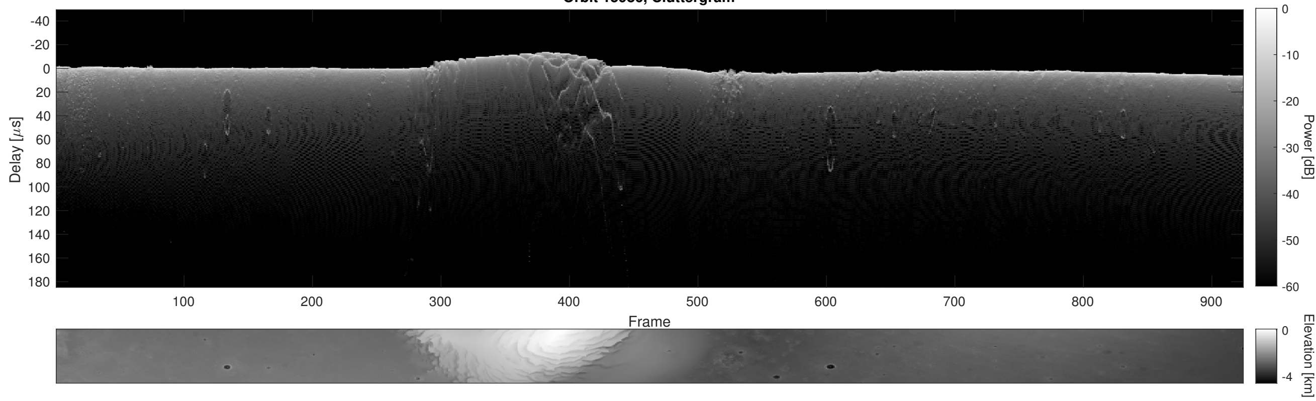
Orbit 15986, Cluttergram
