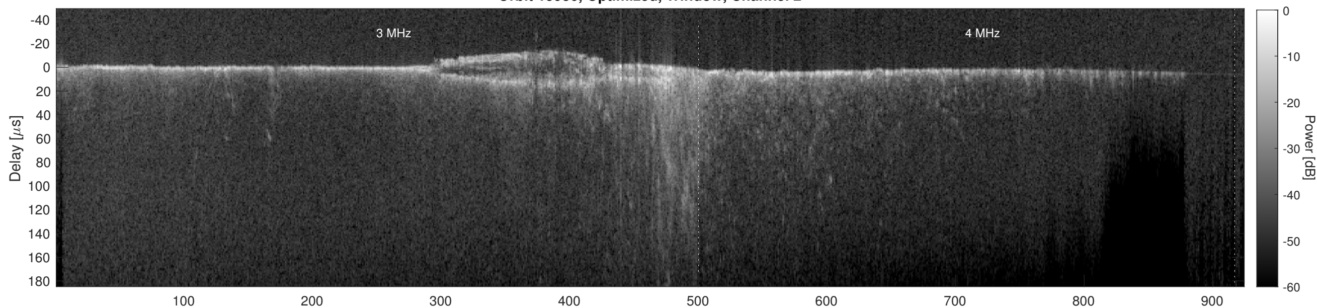
Orbit 15986, Cluttergram
