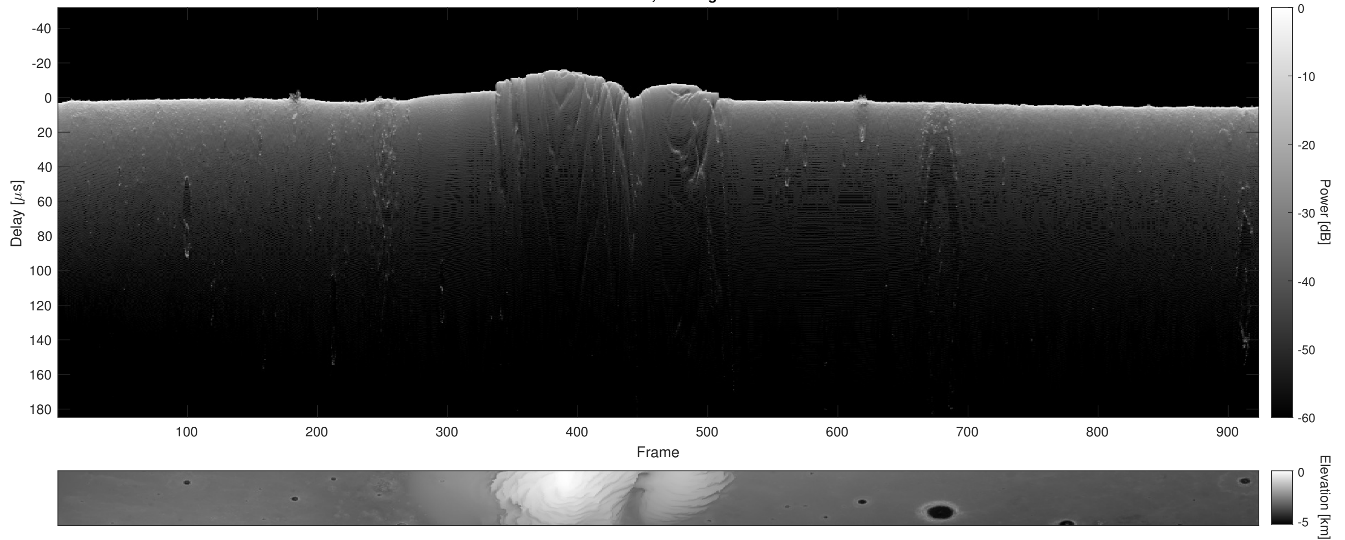
Orbit 15988, Cluttergram
