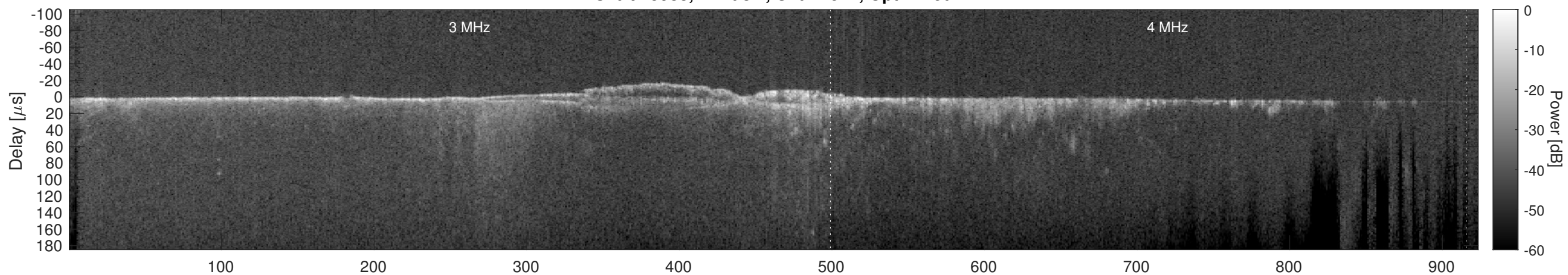
Orbit 15988, Cluttergram
