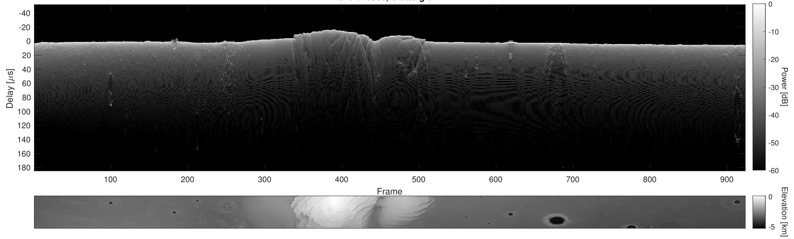
Orbit 15988, Cluttergram
