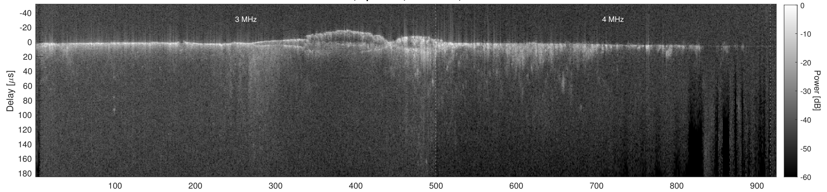
Orbit 15988, Cluttergram
