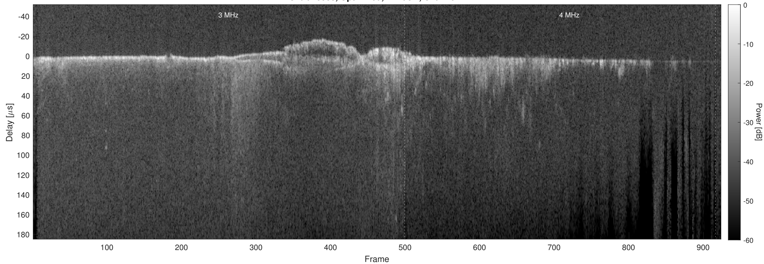
Orbit 15988, Optimized, Window, Channel 2
