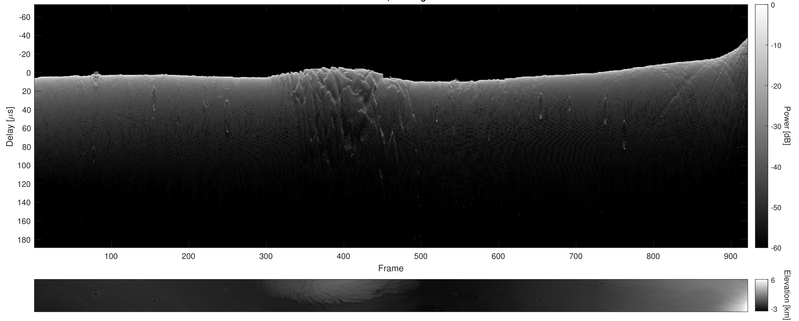
Orbit 15989, Cluttergram
