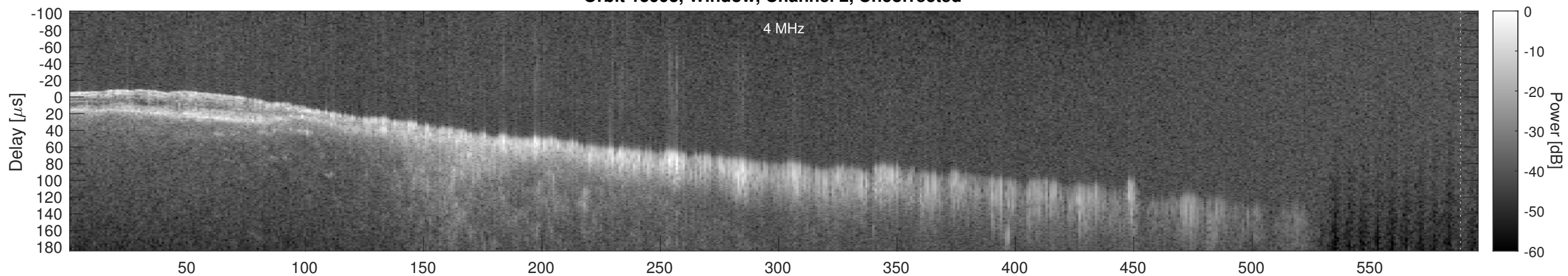
Orbit 15993, Window, Channel 2, Chapman
