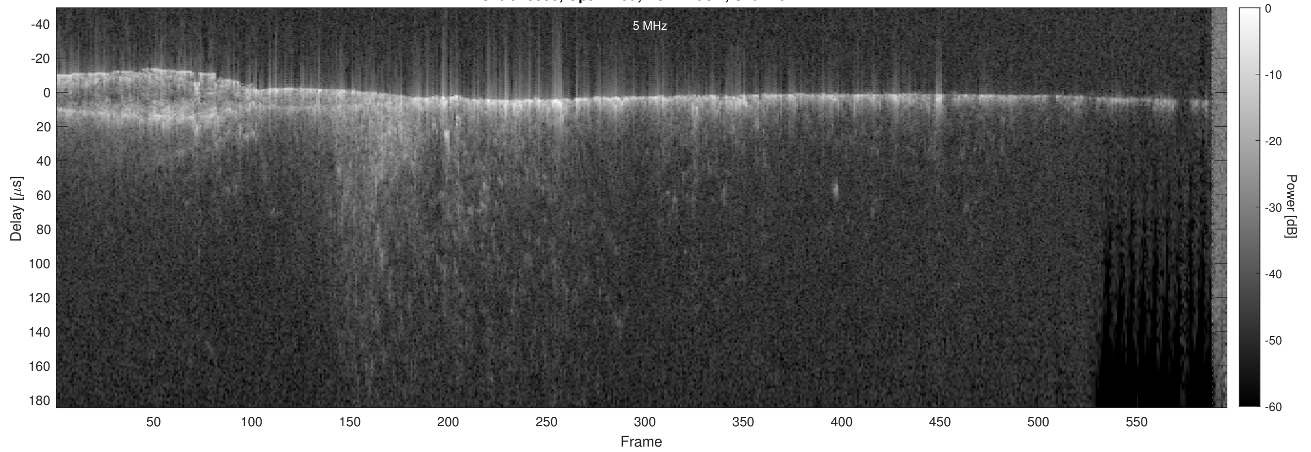
Orbit 15993, Optimized, No Window, Channel 2
