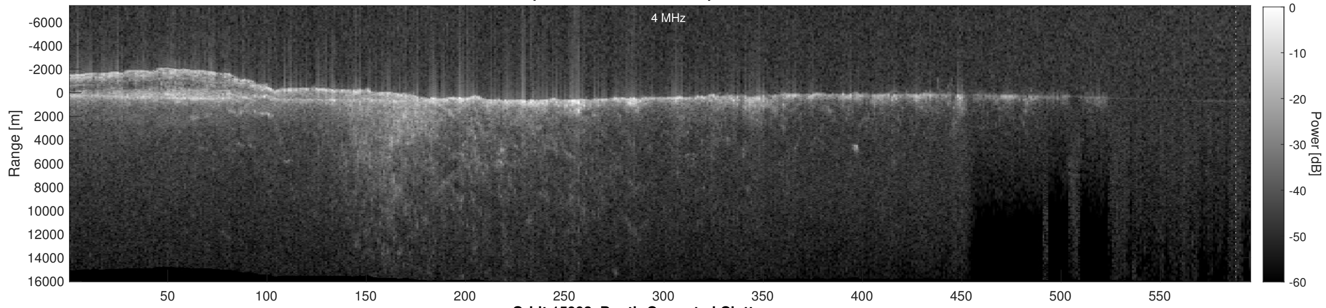
Orbit 15993, Depth-Corrected Cluttergram
