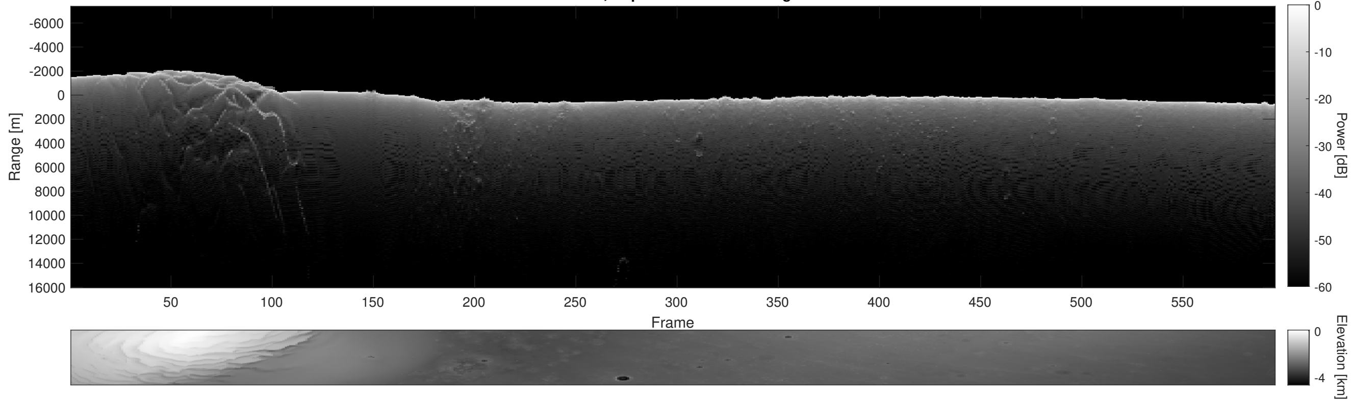
Orbit 15993, Depth-Corrected Cluttergram
