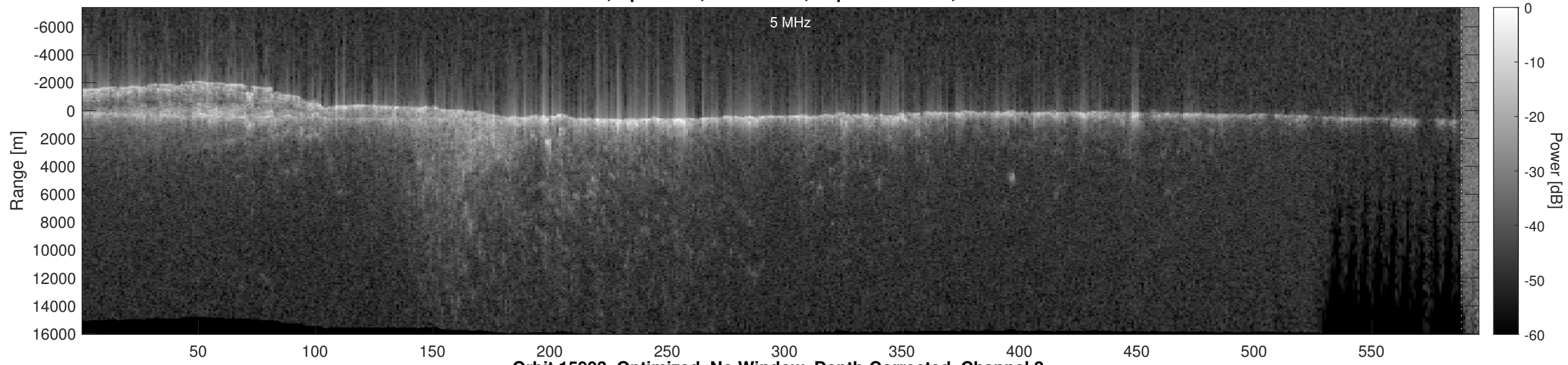
Orbit 15993, Optimized, No Window, Depth-Corrected, Channel 2
