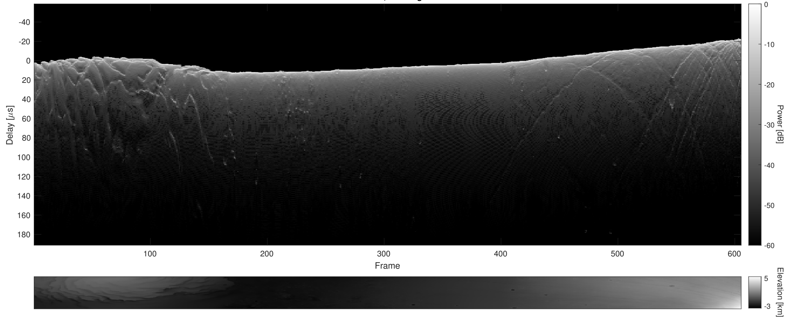
Orbit 15996, Cluttergram
