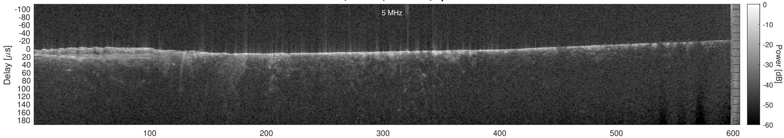
Orbit 15996, Cluttergram
