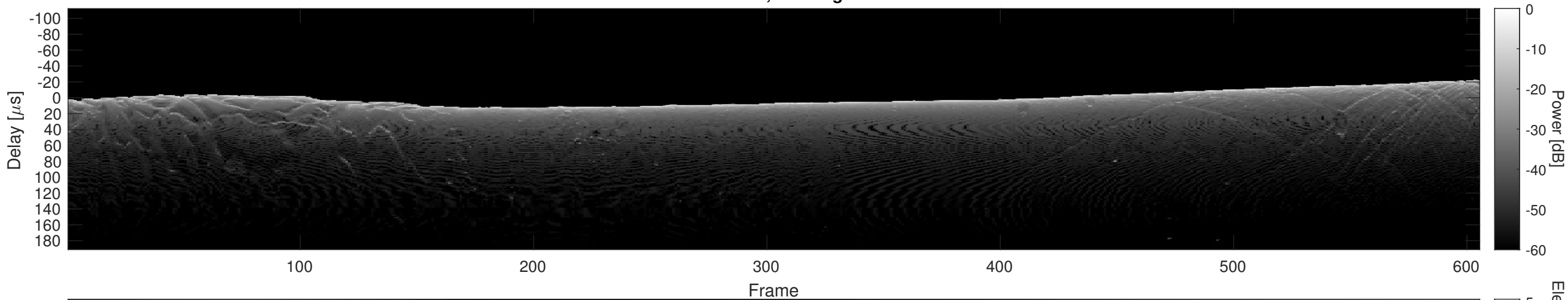
Orbit 15996, Cluttergram
