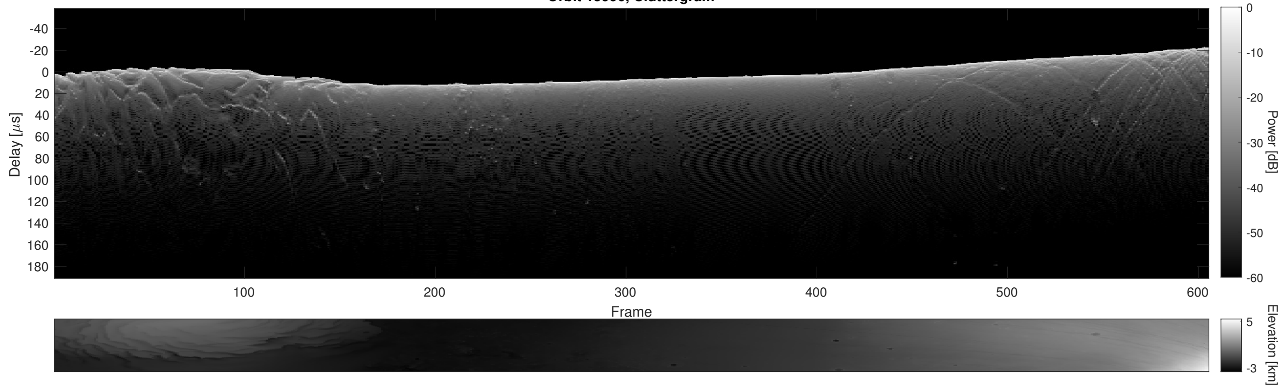
Orbit 15996, Cluttergram
