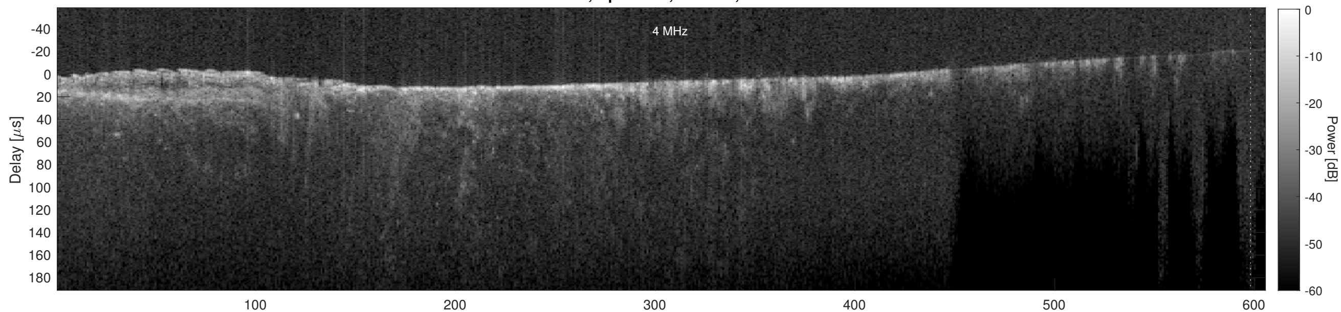
Orbit 15996, Cluttergram
