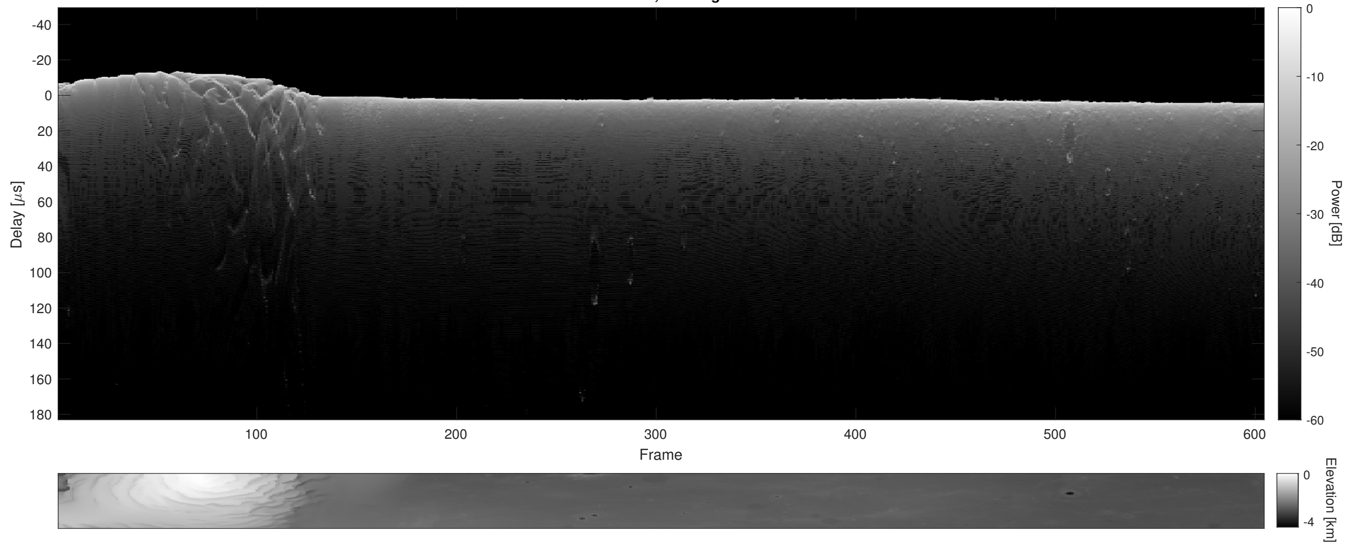
Orbit 15997, Cluttergram
