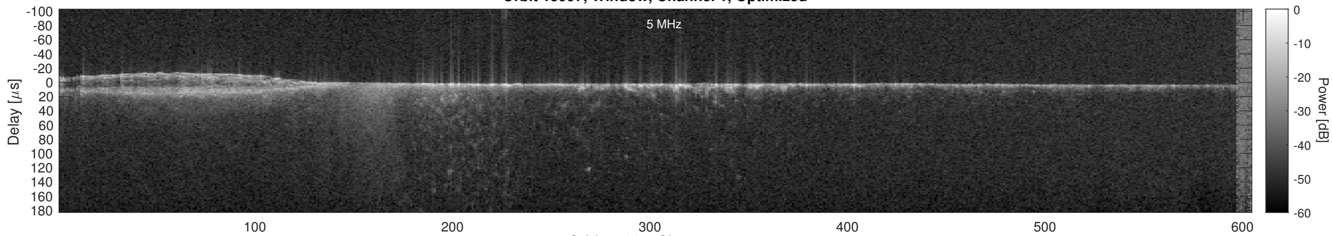
Orbit 15997, Cluttergram
