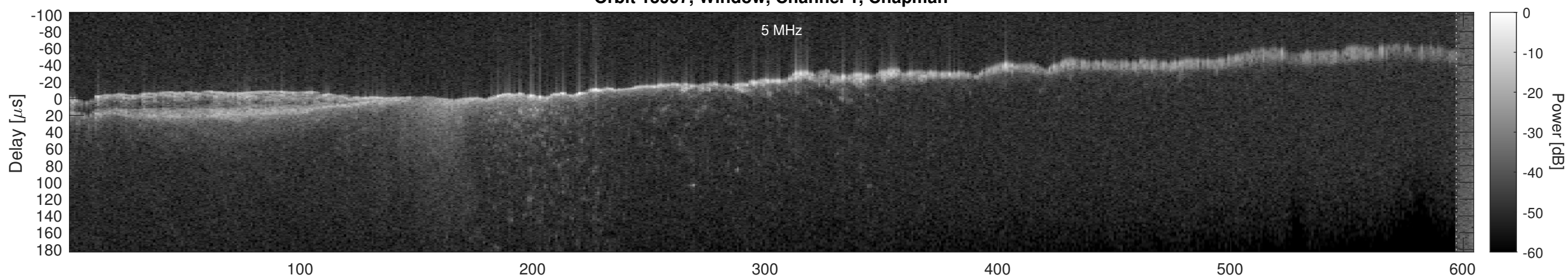
Orbit 15997, Window, Channel 1, Optimized
