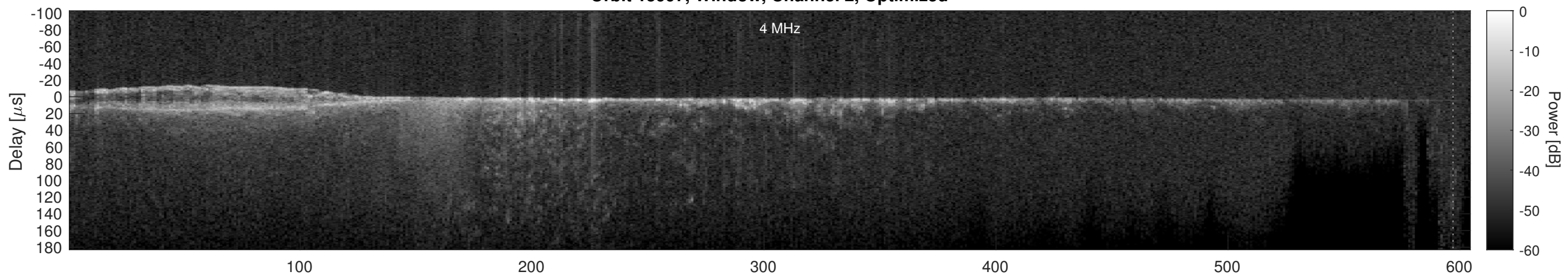
Orbit 15997, Cluttergram
