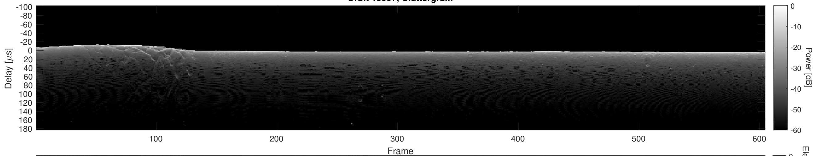
Orbit 15997, Cluttergram
