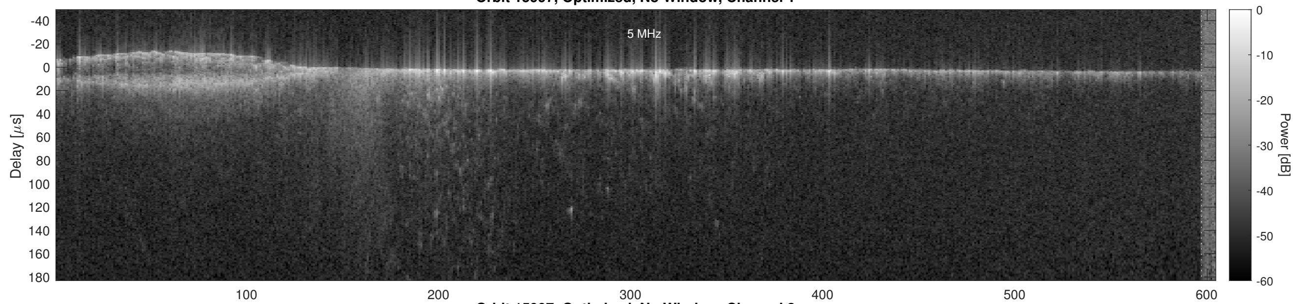
Orbit 15997, Optimized, No Window, Channel 2
