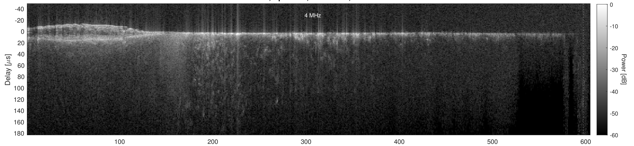
Orbit 15997, Cluttergram
