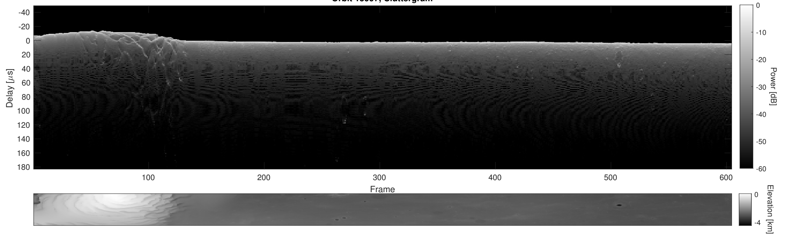
Orbit 15997, Cluttergram
