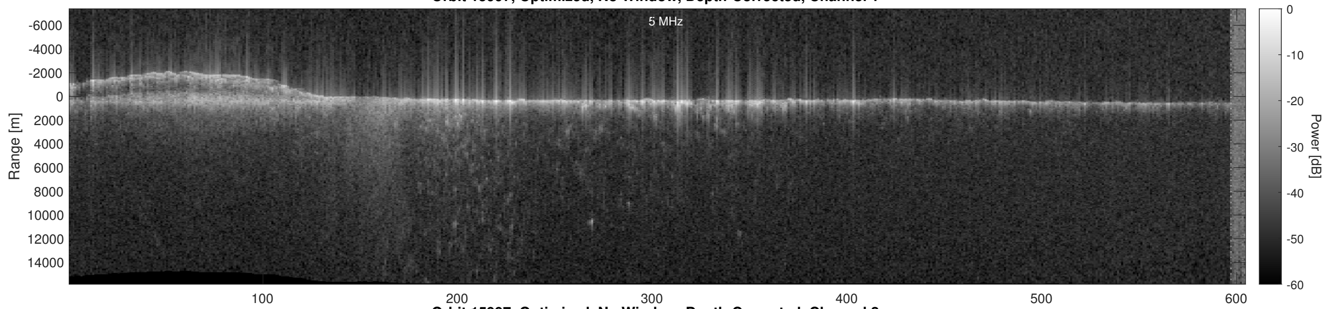
Orbit 15997, Optimized, No Window, Depth-Corrected, Channel 2
