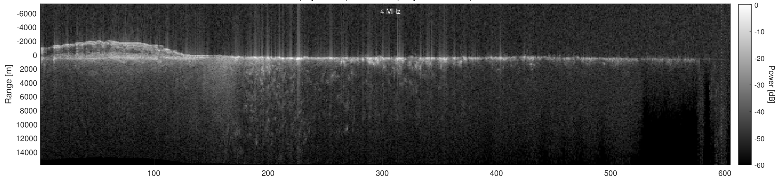
Orbit 15997, Depth-Corrected Cluttergram
