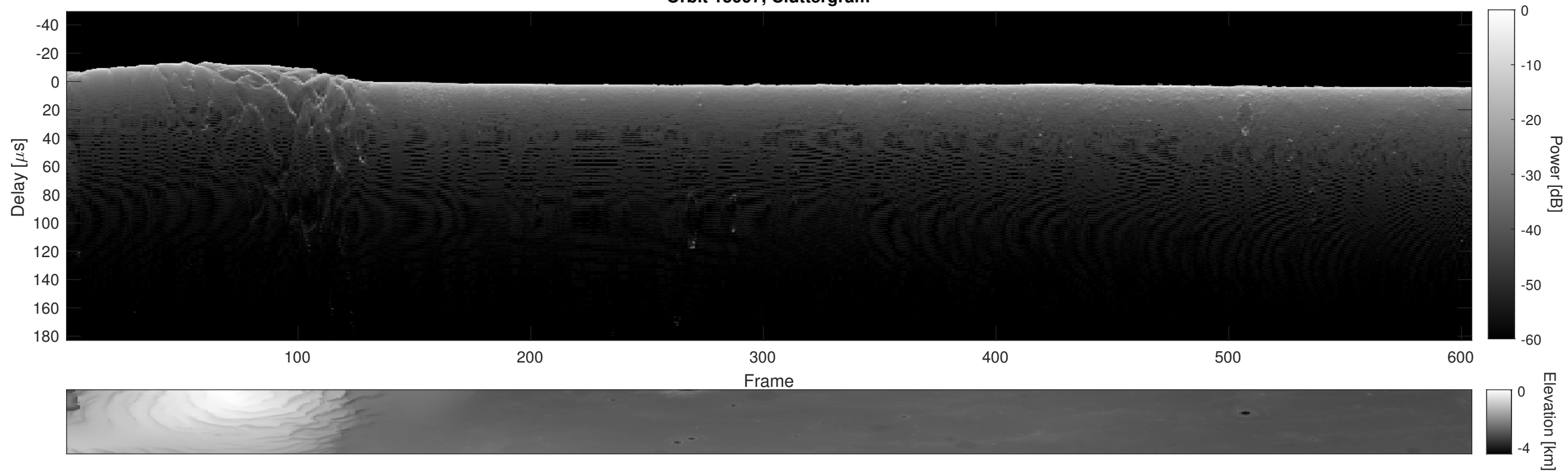
Orbit 15997, Cluttergram
