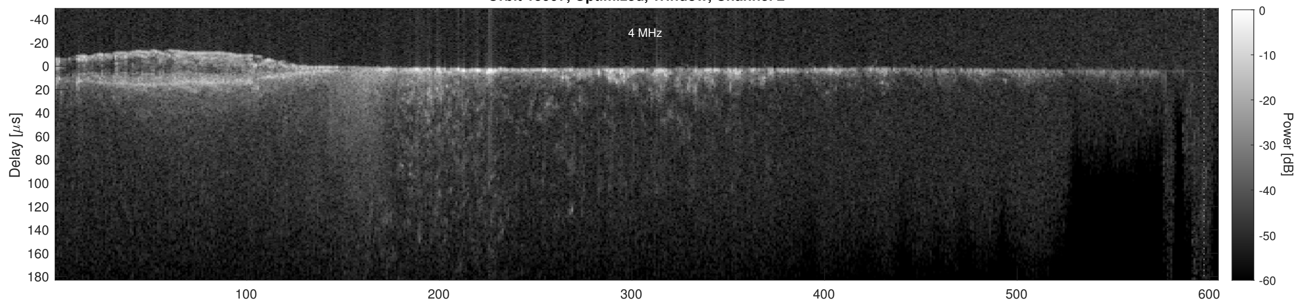
Orbit 15997, Cluttergram
