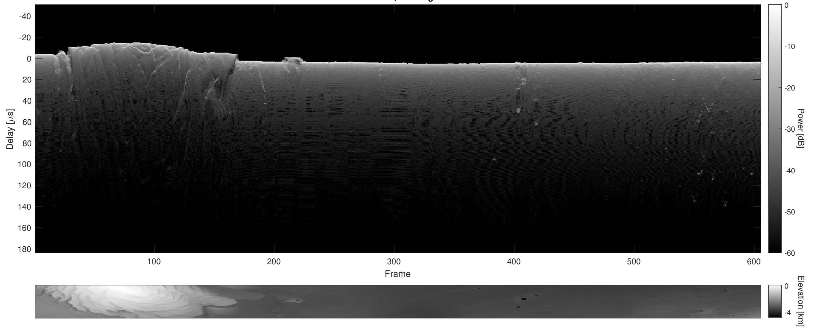
Orbit 15999, Cluttergram
