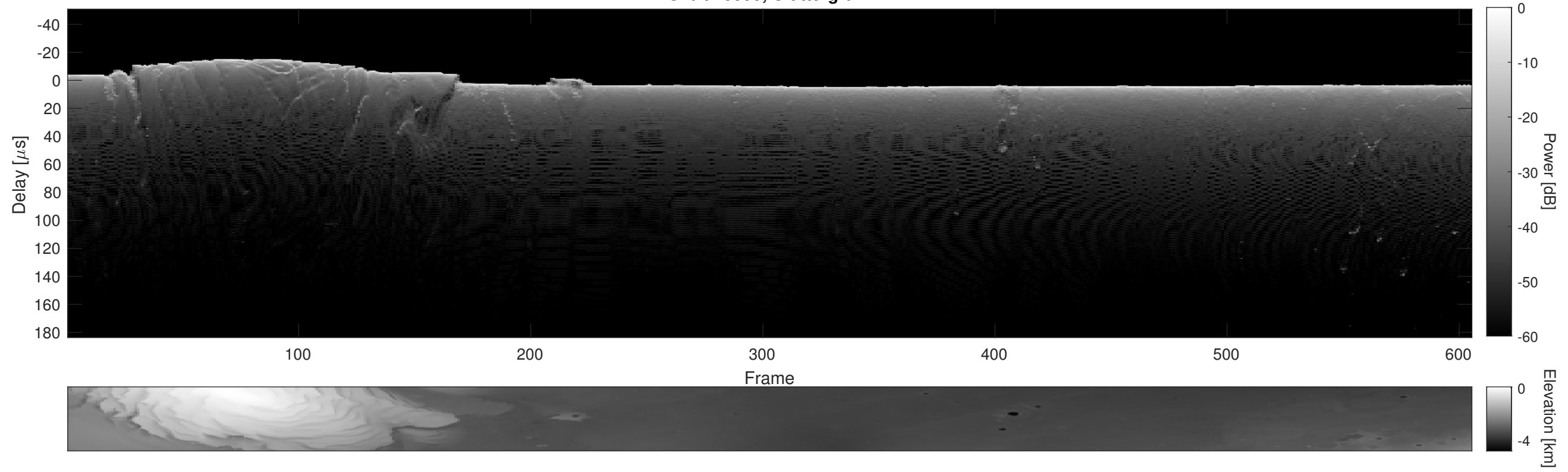
Orbit 15999, Cluttergram
