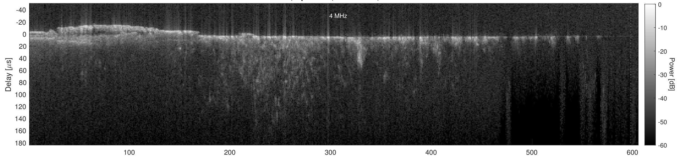
Orbit 15999, Cluttergram
