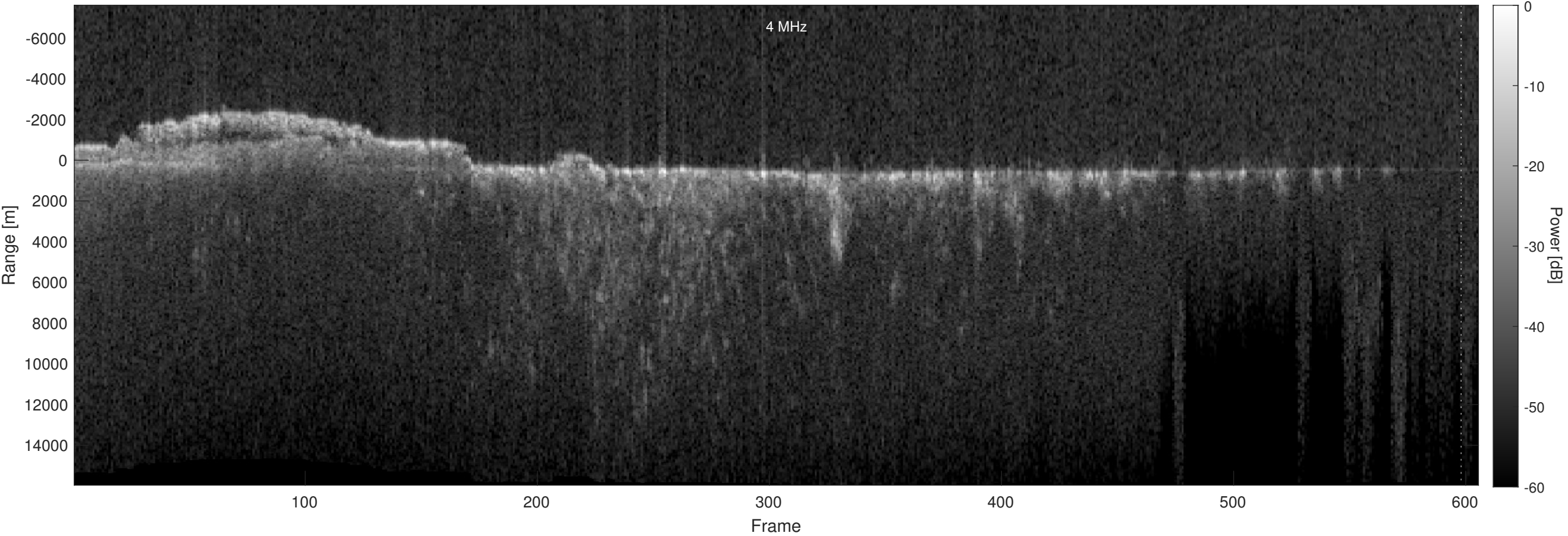
Orbit 15999, Optimized, Window, Depth-Corrected, Channel 2
