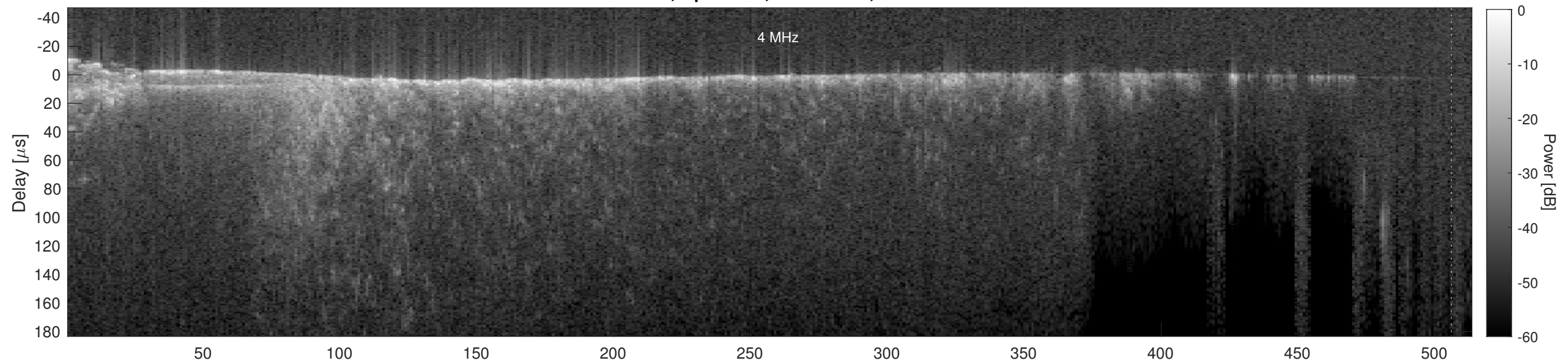
Orbit 16000, Cluttergram
