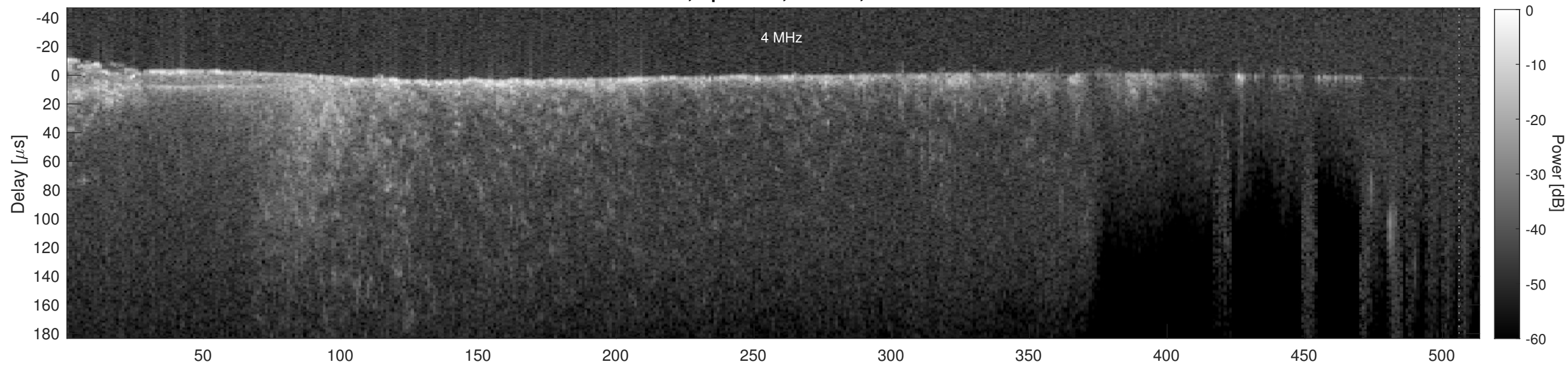
Orbit 16000, Cluttergram
