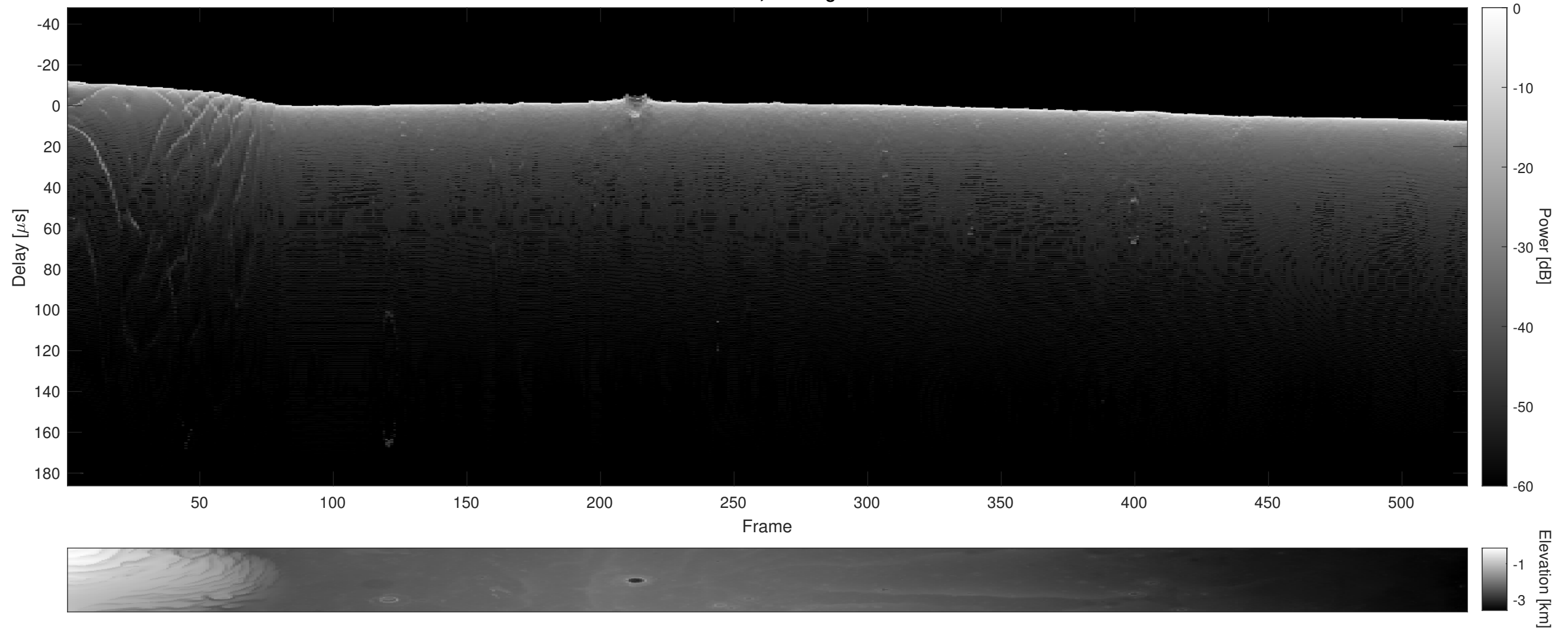
Orbit 16001, Cluttergram
