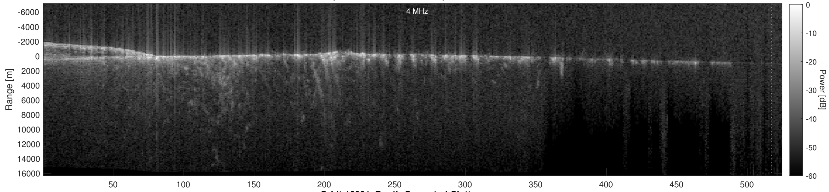
Orbit 16001, Depth-Corrected Cluttergram
