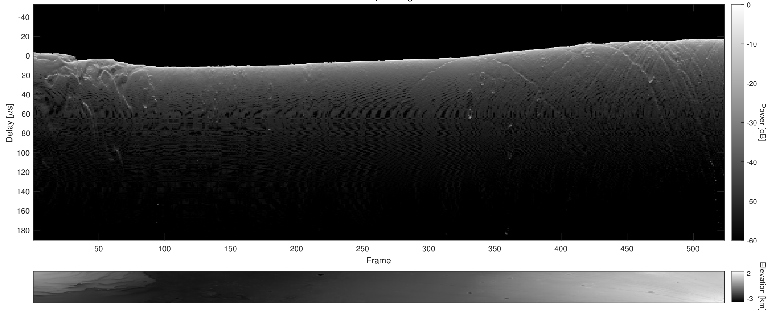
Orbit 16003, Cluttergram
