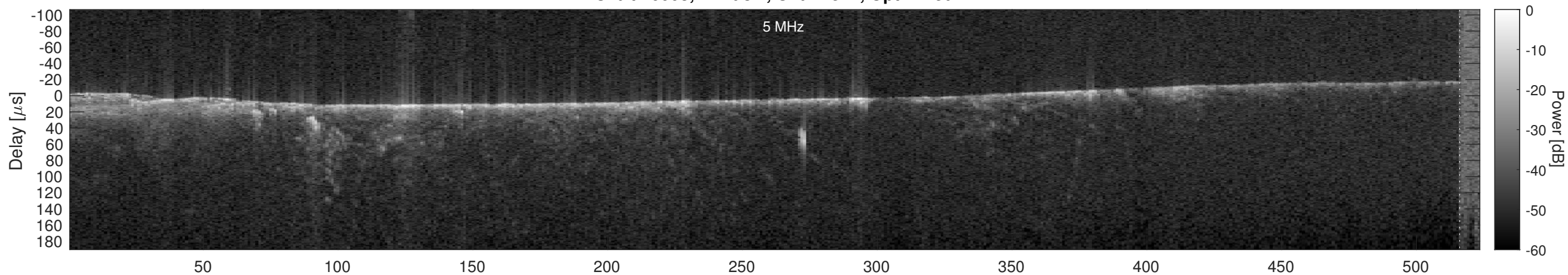
Orbit 16003, Cluttergram
