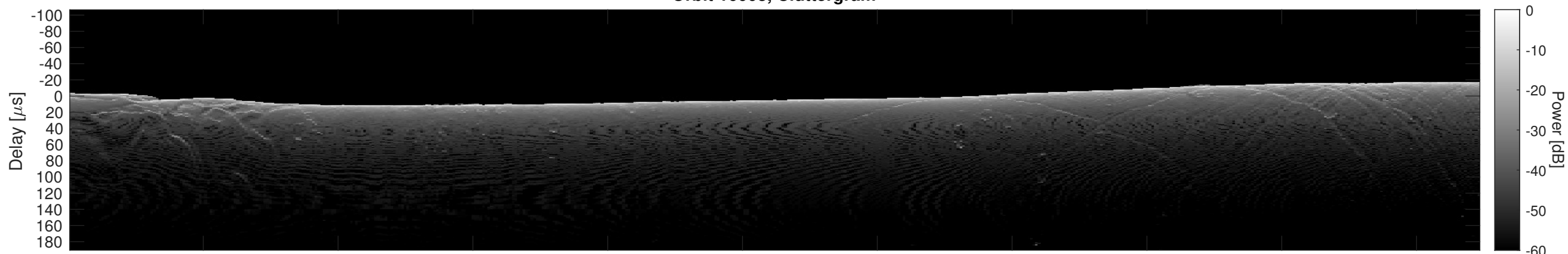
Orbit 16003, Cluttergram
