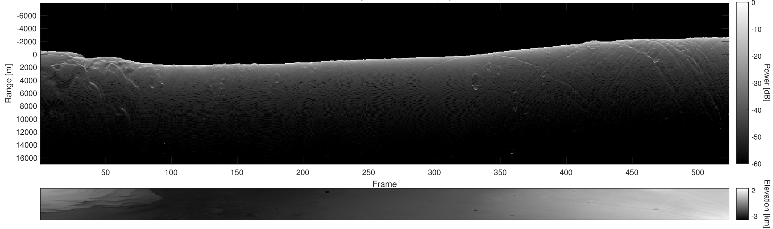
Orbit 16003, Depth-Corrected Cluttergram
