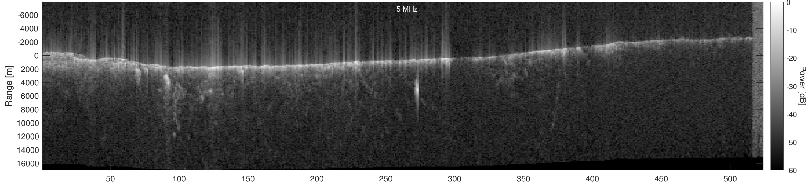
Orbit 16003, Optimized, No Window, Depth-Corrected, Channel 2
