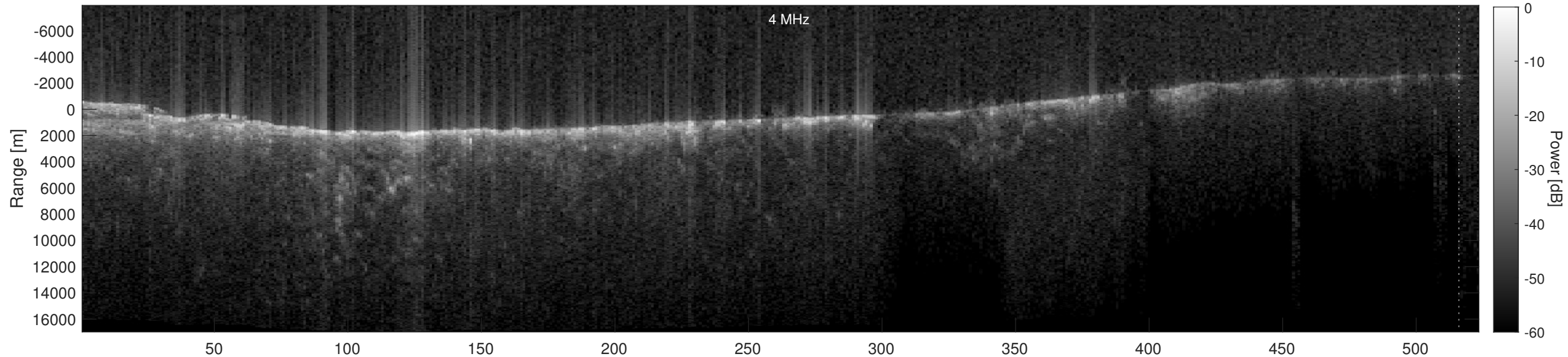
Orbit 16003, Depth-Corrected Cluttergram
