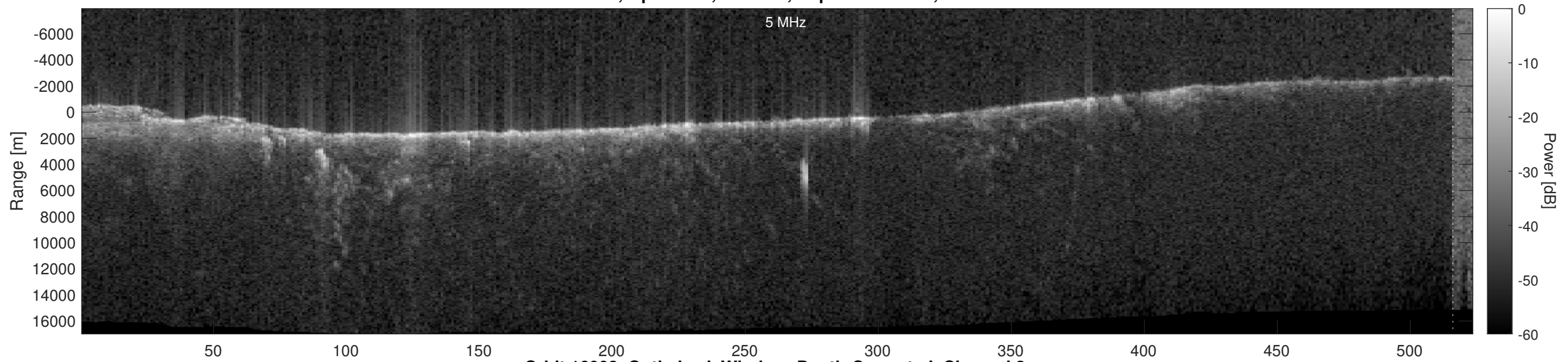
Orbit 16003, Optimized, Window, Depth-Corrected, Channel 2
