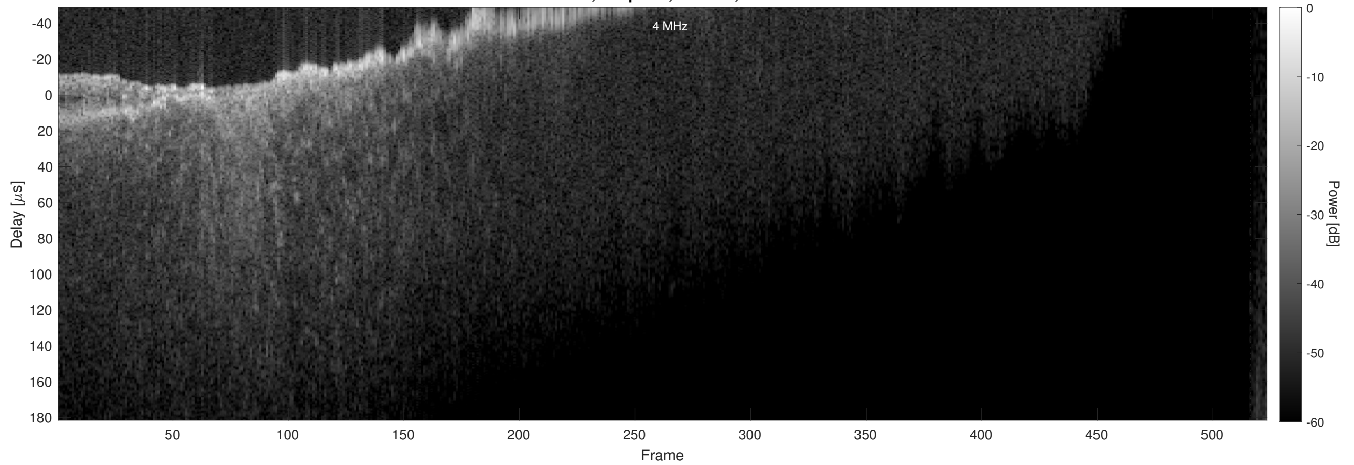
Orbit 16004, Chapman, Window, Channel 2
