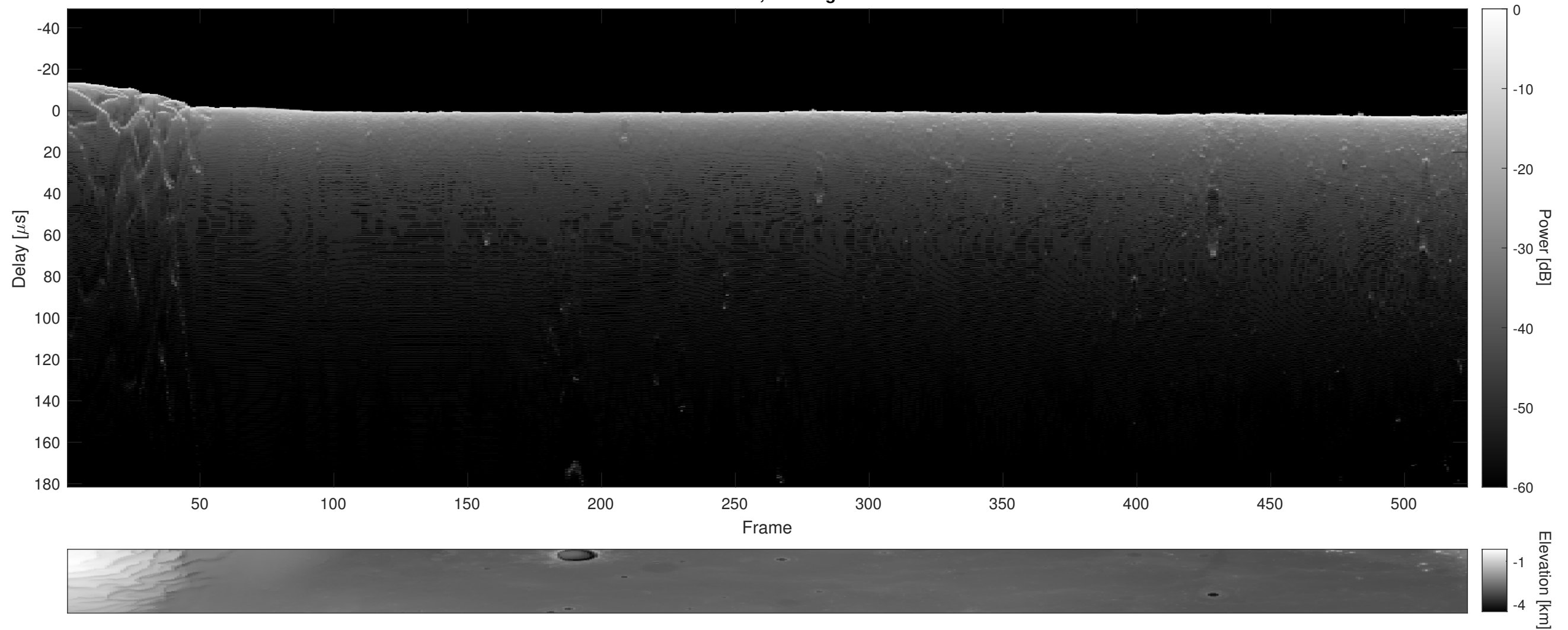
Orbit 16004, Cluttergram
