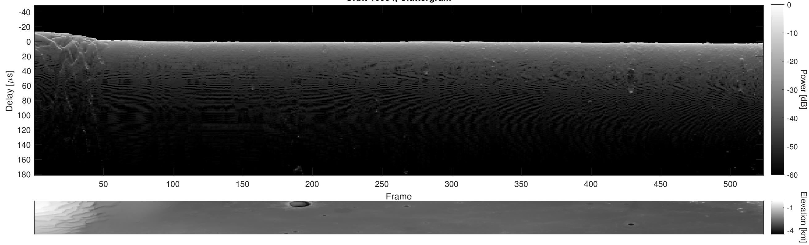
Orbit 16004, Cluttergram
