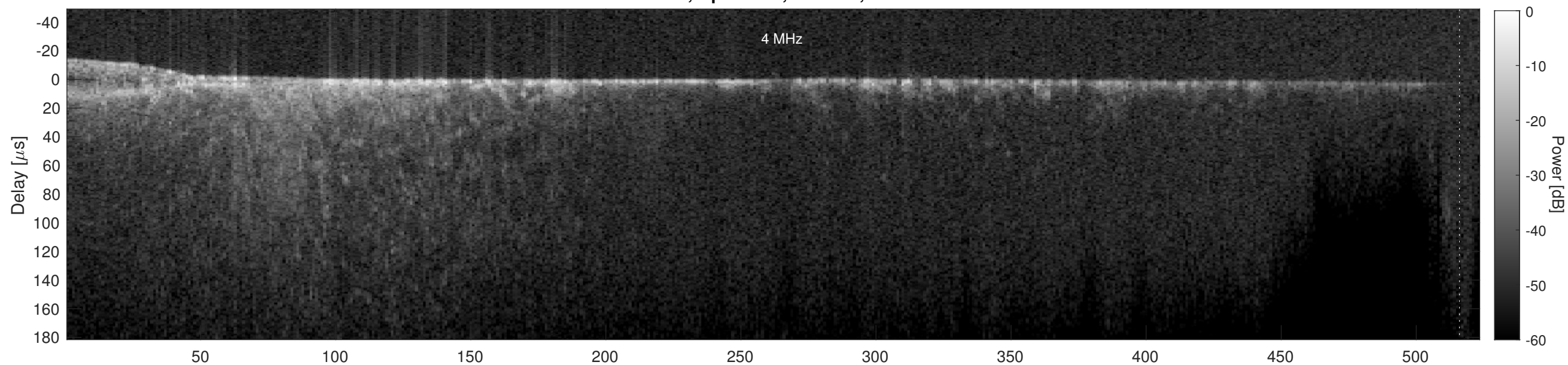
Orbit 16004, Cluttergram
