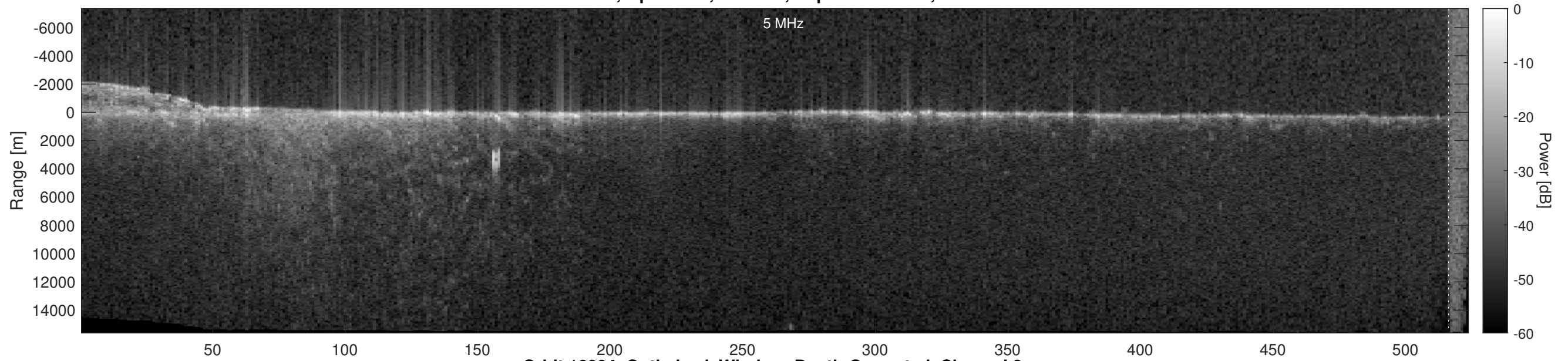
Orbit 16004, Optimized, Window, Depth-Corrected, Channel 2
