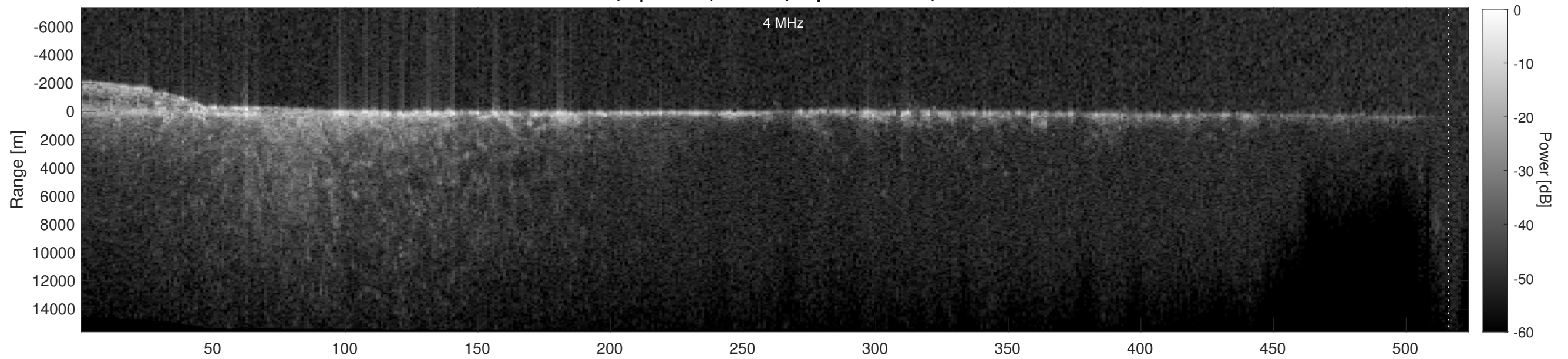
Orbit 16004, Depth-Corrected Cluttergram
