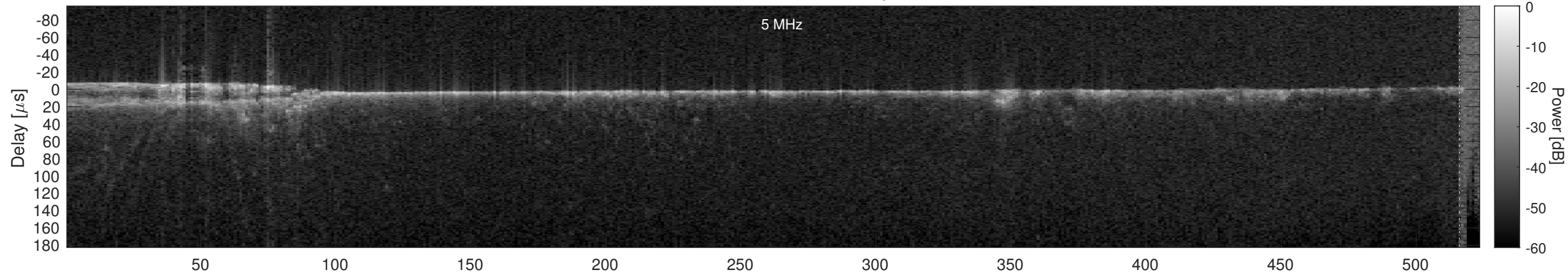
Orbit 16005, Cluttergram
