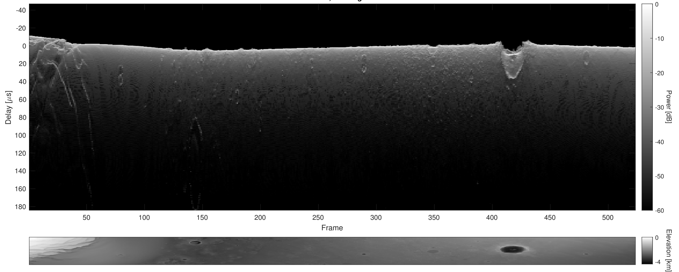
Orbit 16007, Cluttergram
